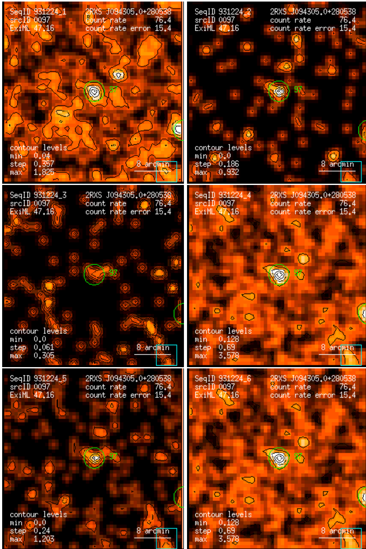
Figure 97: RASS 931224: detection 0097: band rate images, Gaussian filter: (1) PSPC channels 11 – 41, (2) 52 – 90, (3) 91 – 201, (4) 11 – 235, (5) 52 – 201, (6) 11 – 201. Broad band rates in counts/ks. Band rate contour levels in counts/ks/arcmin 2 .
