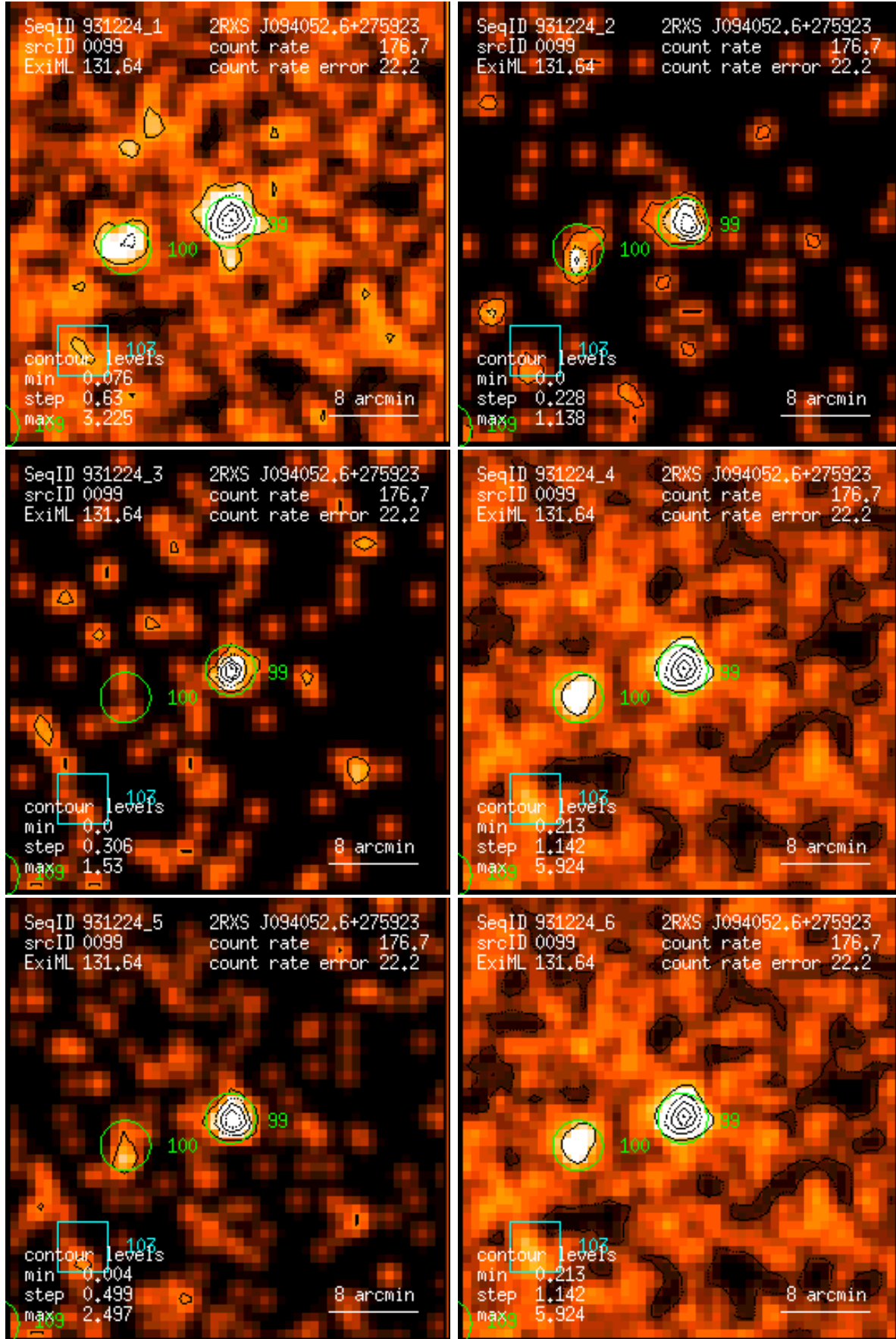
Figure 99: RASS 931224: detection 0099: band rate images, Gaussian filter: (1) PSPC channels 11 – 41, (2) 52 – 90, (3) 91 – 201, (4) 11 – 235, (5) 52 – 201, (6) 11 – 201. Broad band rates in counts/ks. Band rate contour levels in counts/ks/arcmin 2 .
