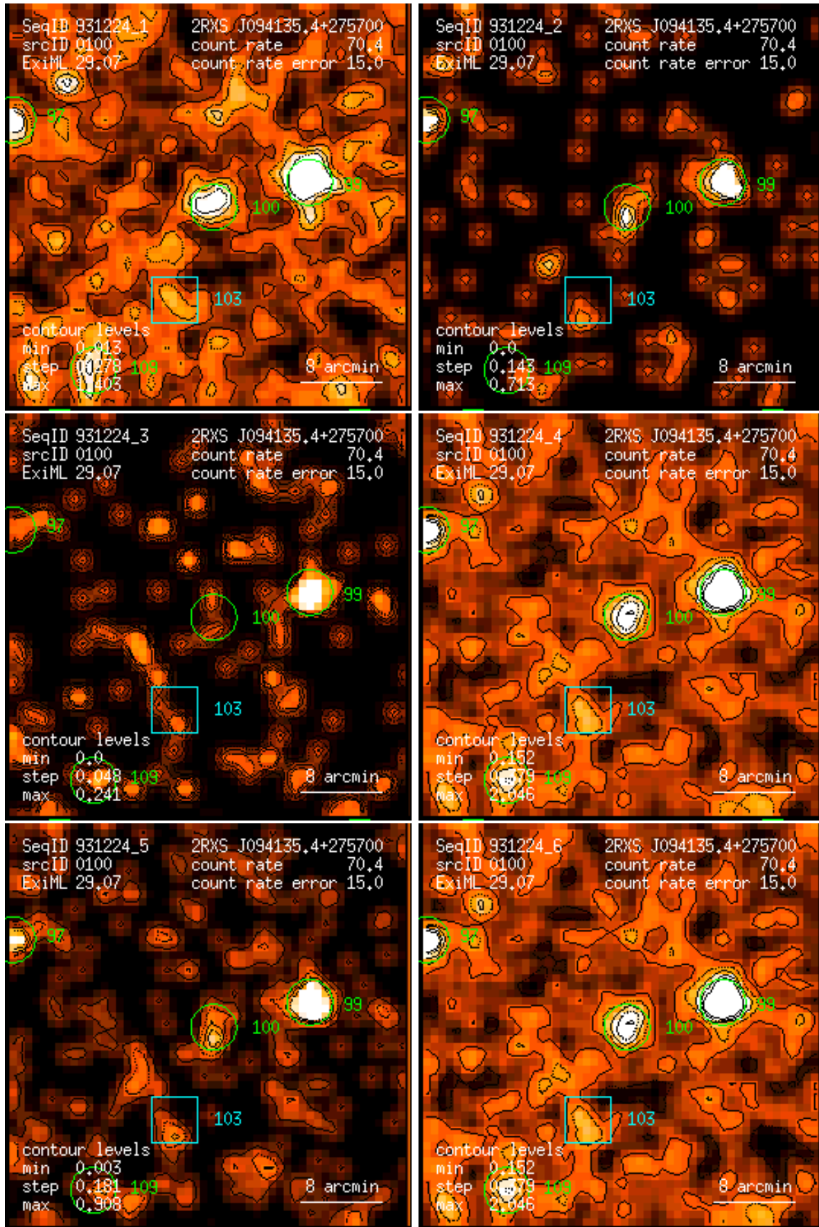
Figure 100: RASS 931224: detection 0100: band rate images, Gaussian filter: (1) PSPC channels 11 – 41, (2) 52 – 90, (3) 91 – 201, (4) 11 – 235, (5) 52 – 201, (6) 11 – 201. Broad band rates in counts/ks. Band rate contour levels in counts/ks/arcmin 2 .
