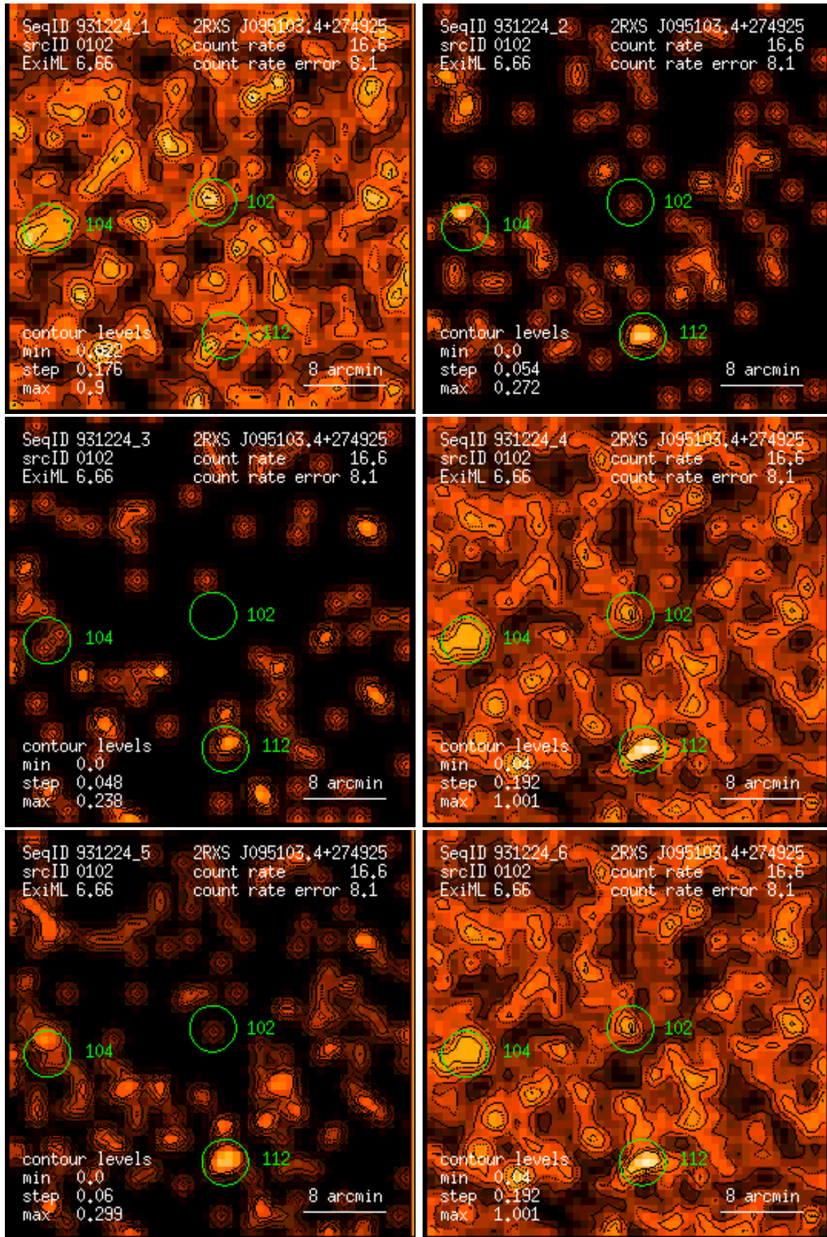
Figure 102: RASS 931224: detection 0102: band rate images, Gaussian filter: (1) PSPC channels 11 – 41, (2) 52 – 90, (3) 91 – 201, (4) 11 – 235, (5) 52 – 201, (6) 11 – 201. Broad band rates in counts/ks. Band rate contour levels in counts/ks/arcmin 2 .
