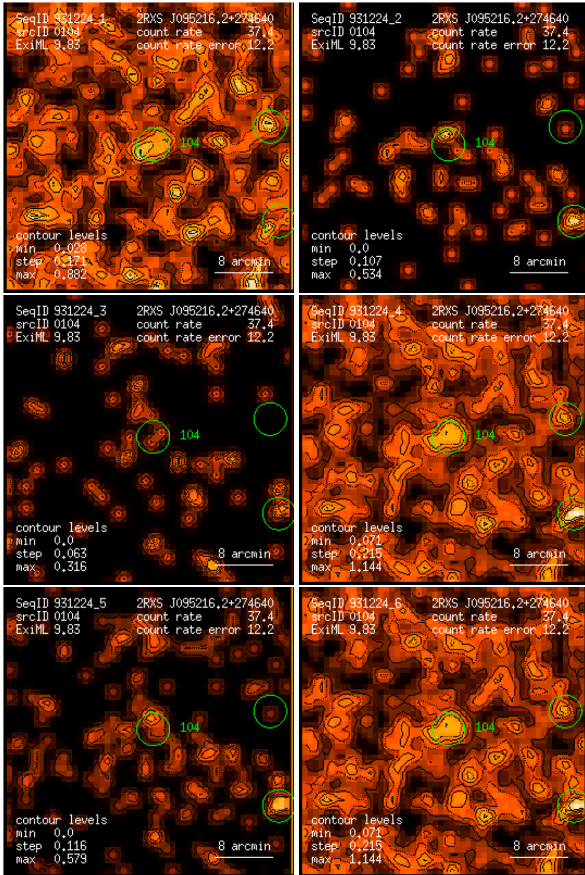
Figure 104: RASS 931224: detection 0104: band rate images, Gaussian filter: (1) PSPC channels 11 – 41, (2) 52 – 90, (3) 91 – 201, (4) 11 – 235, (5) 52 – 201, (6) 11 – 201. Broad band rates in counts/ks. Band rate contour levels in counts/ks/arcmin 2 .
