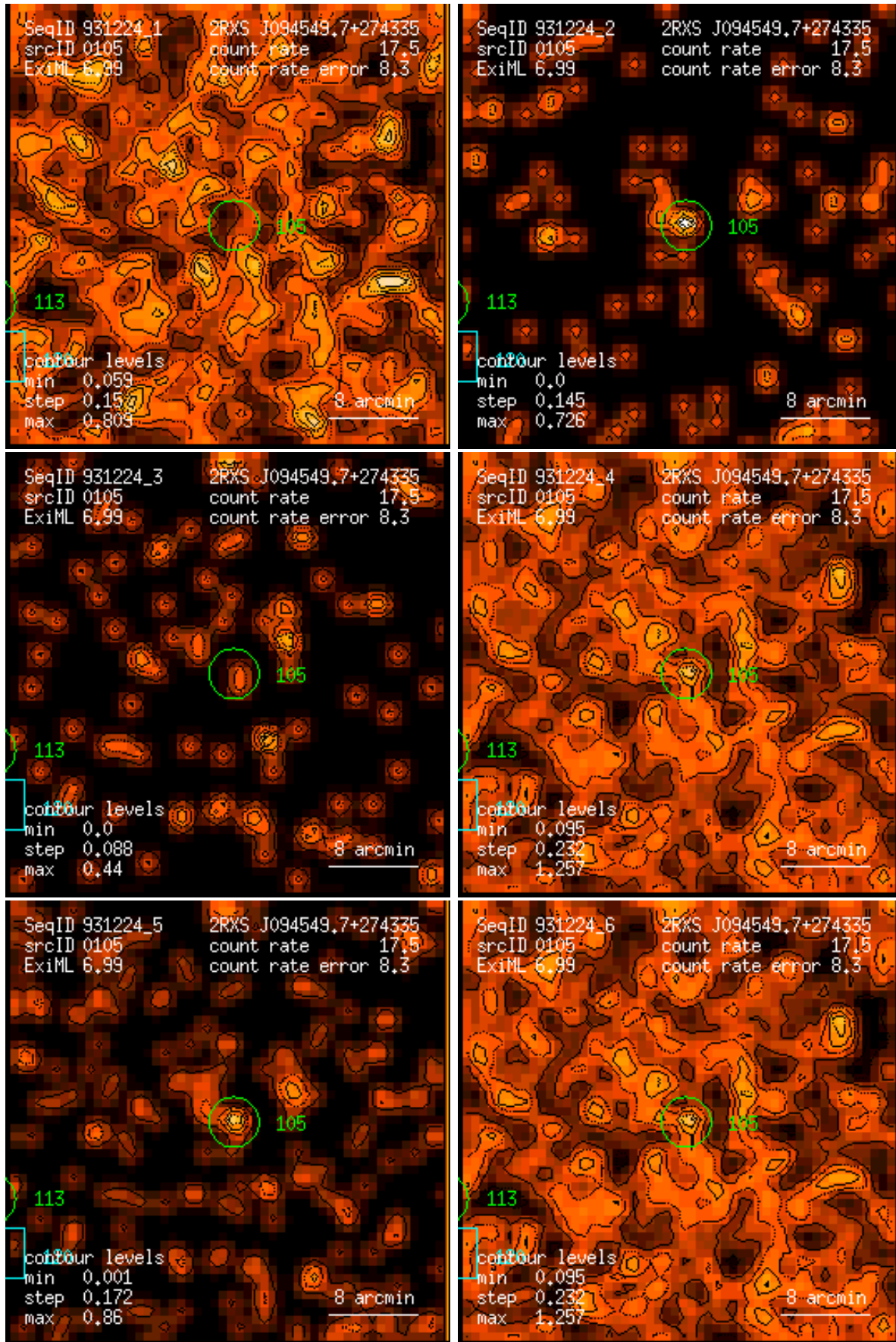
Figure 105: RASS 931224: detection 0105: band rate images, Gaussian filter: (1) PSPC channels 11 – 41, (2) 52 – 90, (3) 91 – 201, (4) 11 – 235, (5) 52 – 201, (6) 11 – 201. Broad band rates in counts/ks. Band rate contour levels in counts/ks/arcmin 2 .
