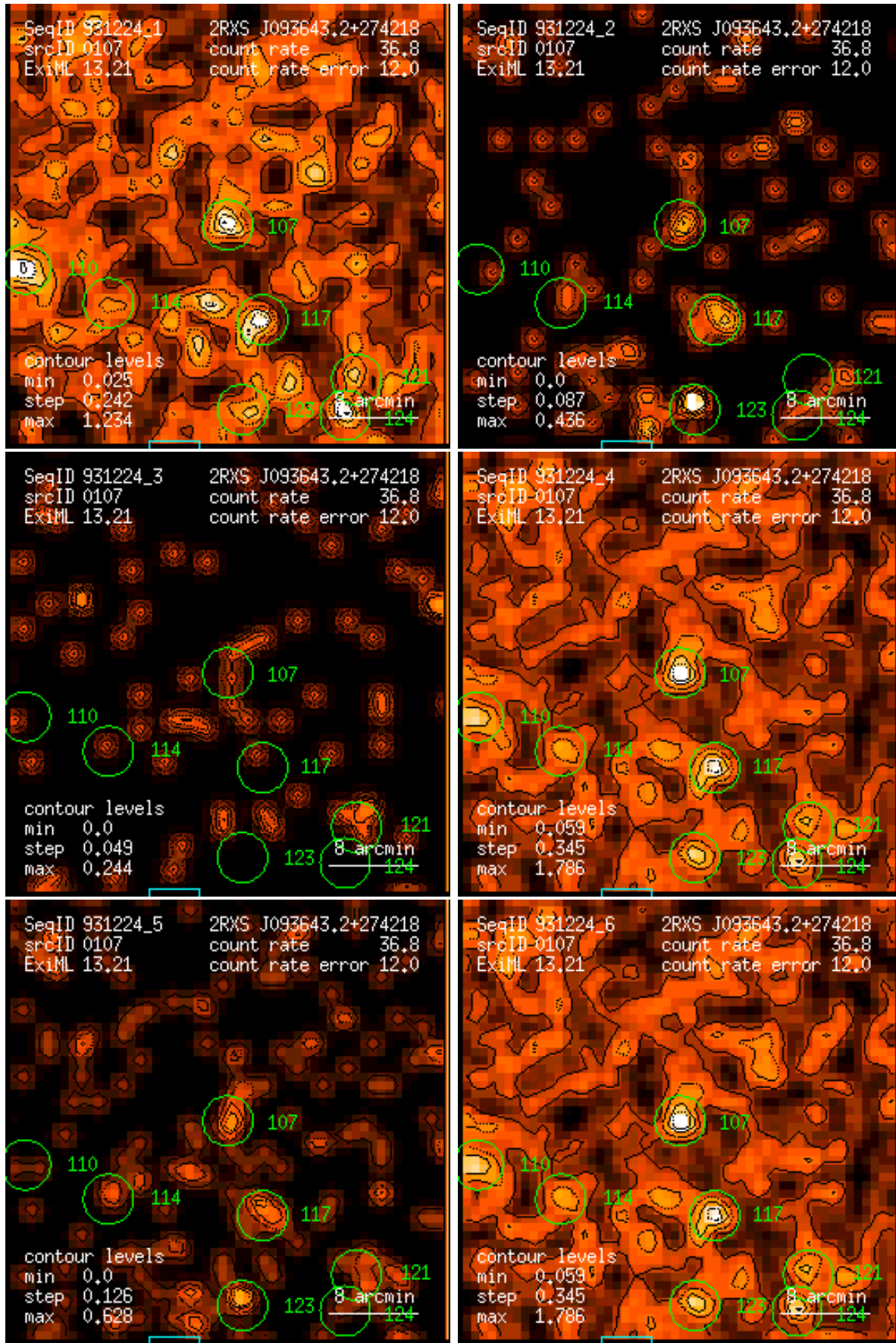
Figure 107: RASS 931224: detection 0107: band rate images, Gaussian filter: (1) PSPC channels 11 – 41, (2) 52 – 90, (3) 91 – 201, (4) 11 – 235, (5) 52 – 201, (6) 11 – 201. Broad band rates in counts/ks. Band rate contour levels in counts/ks/arcmin 2 .
