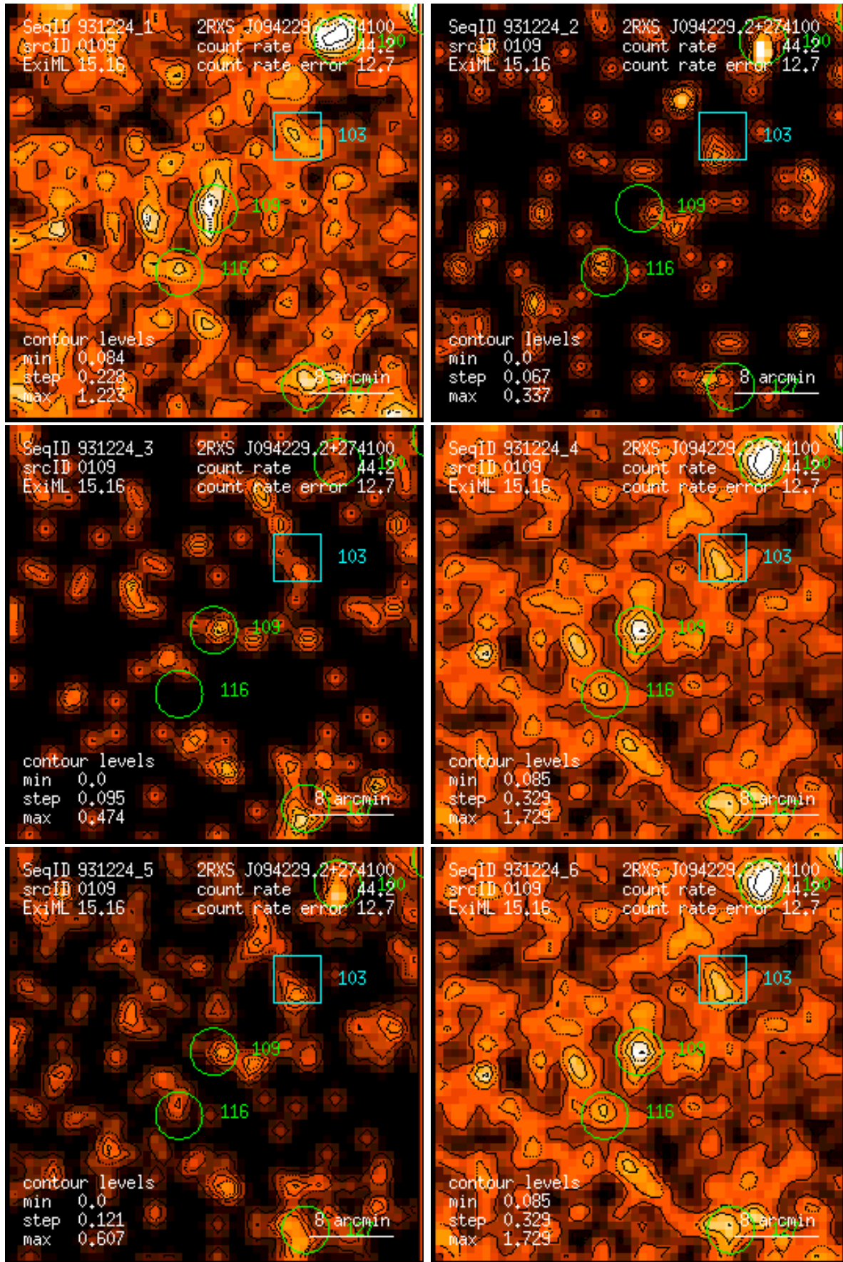
Figure 109: RASS 931224: detection 0109: band rate images, Gaussian filter: (1) PSPC channels 11 – 41, (2) 52 – 90, (3) 91 – 201, (4) 11 – 235, (5) 52 – 201, (6) 11 – 201. Broad band rates in counts/ks. Band rate contour levels in counts/ks/arcmin 2 .
