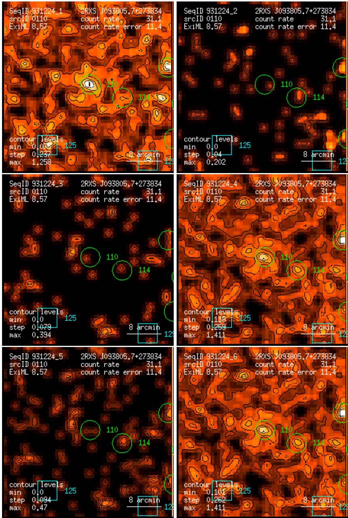
Figure 110: RASS 931224: detection 0110: band rate images, Gaussian filter: (1) PSPC channels 11 – 41, (2) 52 – 90, (3) 91 – 201, (4) 11 – 235, (5) 52 – 201, (6) 11 – 201. Broad band rates in counts/ks. Band rate contour levels in counts/ks/arcmin 2 .
