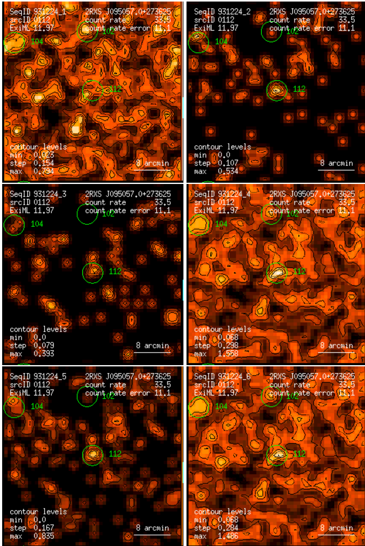
Figure 112: RASS 931224: detection 0112: band rate images, Gaussian filter: (1) PSPC channels 11 – 41, (2) 52 – 90, (3) 91 – 201, (4) 11 – 235, (5) 52 – 201, (6) 11 – 201. Broad band rates in counts/ks. Band rate contour levels in counts/ks/arcmin 2 .
