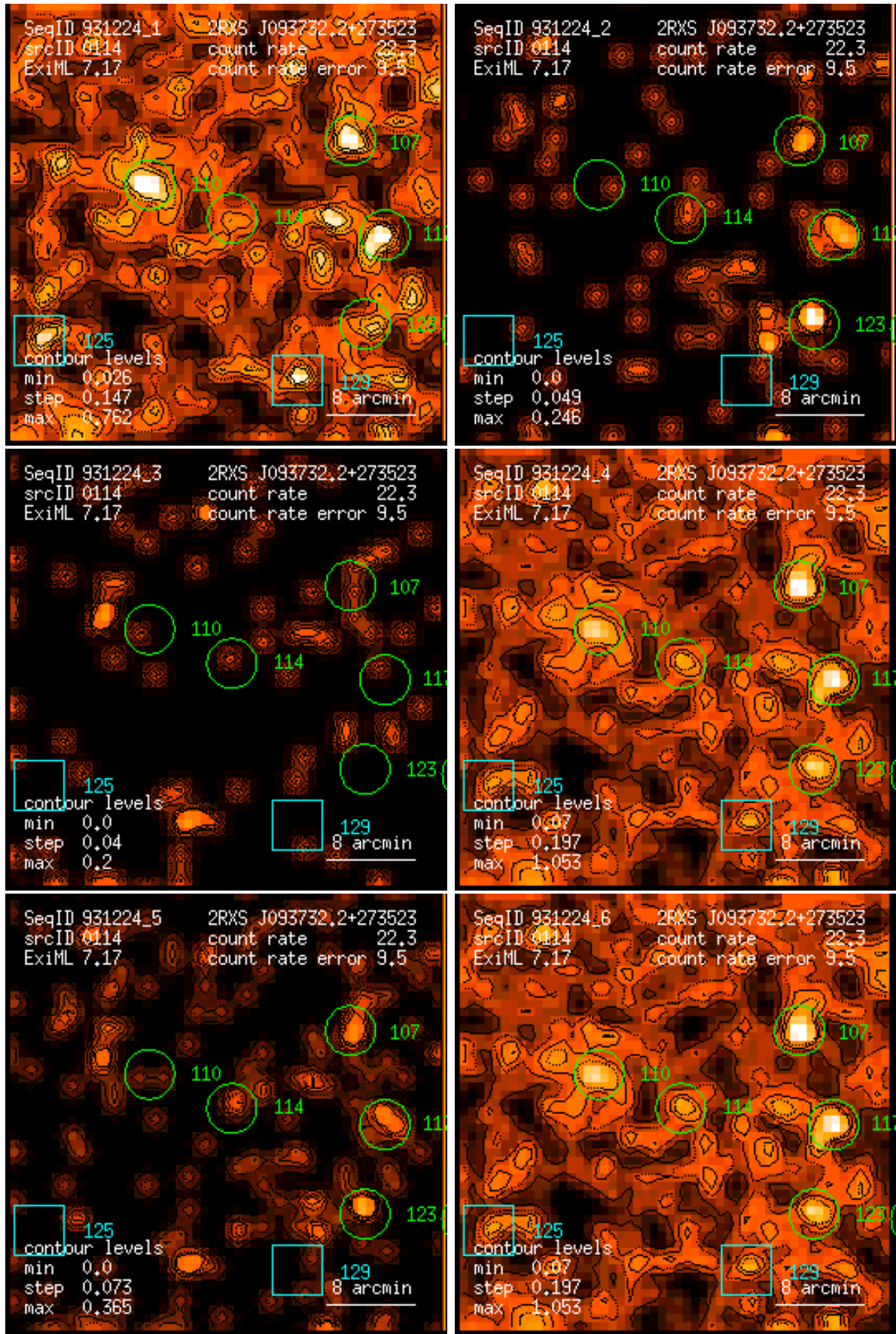
Figure 114: RASS 931224: detection 0114: band rate images, Gaussian filter: (1) PSPC channels 11 – 41, (2) 52 – 90, (3) 91 – 201, (4) 11 – 235, (5) 52 – 201, (6) 11 – 201. Broad band rates in counts/ks. Band rate contour levels in counts/ks/arcmin 2 .
