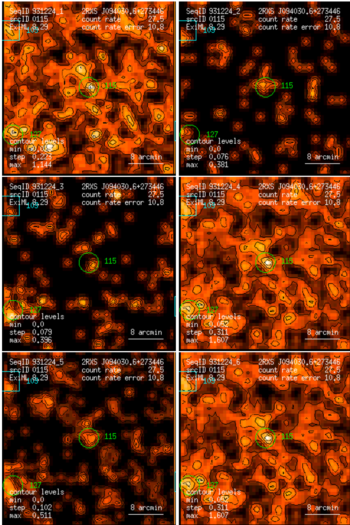
Figure 115: RASS 931224: detection 0115: band rate images, Gaussian filter: (1) PSPC channels 11 – 41, (2) 52 – 90, (3) 91 – 201, (4) 11 – 235, (5) 52 – 201, (6) 11 – 201. Broad band rates in counts/ks. Band rate contour levels in counts/ks/arcmin 2 .
