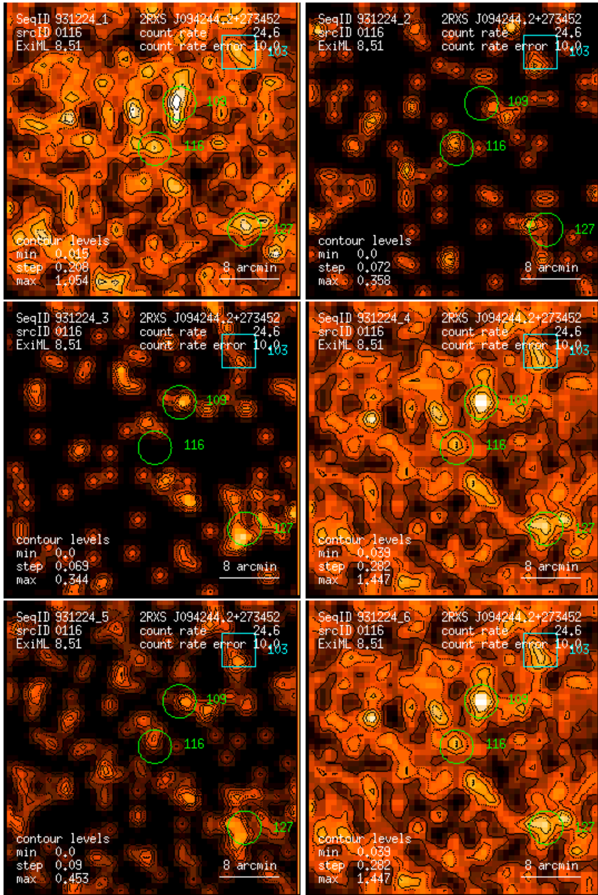
Figure 116: RASS 931224: detection 0116: band rate images, Gaussian filter: (1) PSPC channels 11 – 41, (2) 52 – 90, (3) 91 – 201, (4) 11 – 235, (5) 52 – 201, (6) 11 – 201. Broad band rates in counts/ks. Band rate contour levels in counts/ks/arcmin 2 .
