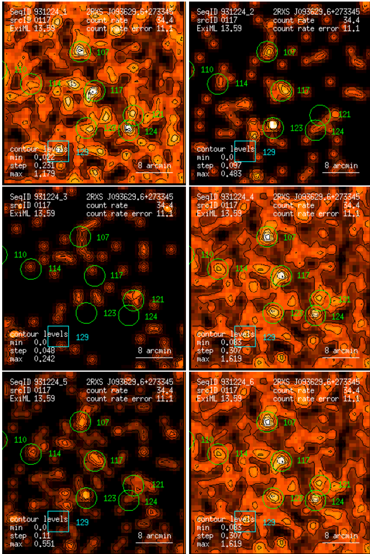
Figure 117: RASS 931224: detection 0117: band rate images, Gaussian filter: (1) PSPC channels 11 – 41, (2) 52 – 90, (3) 91 – 201, (4) 11 – 235, (5) 52 – 201, (6) 11 – 201. Broad band rates in counts/ks. Band rate contour levels in counts/ks/arcmin 2 .
