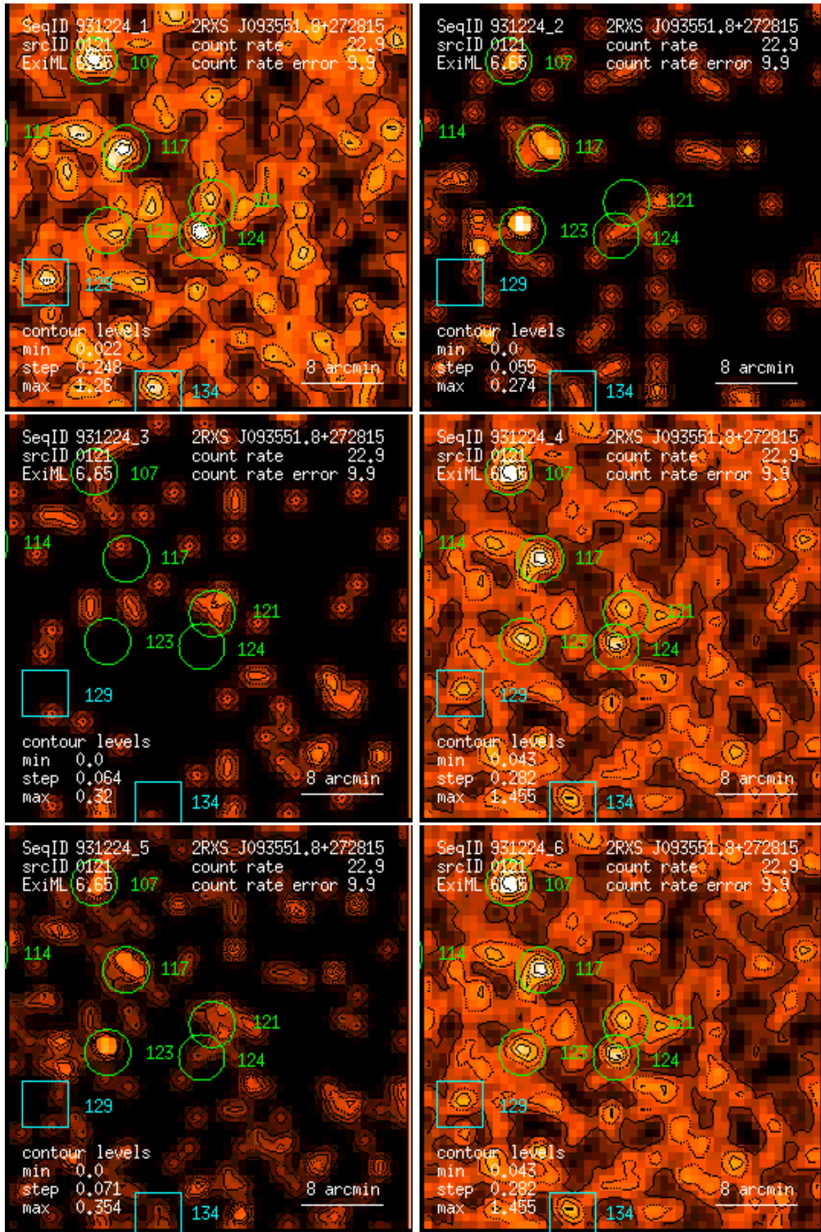
Figure 121: RASS 931224: detection 0121: band rate images, Gaussian filter: (1) PSPC channels 11 – 41, (2) 52 – 90, (3) 91 – 201, (4) 11 – 235, (5) 52 – 201, (6) 11 – 201. Broad band rates in counts/ks. Band rate contour levels in counts/ks/arcmin 2 .
