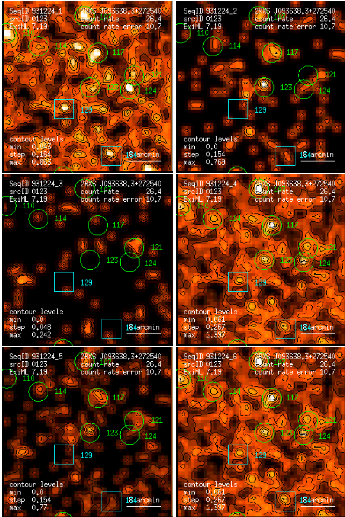
Figure 123: RASS 931224: detection 0123: band rate images, Gaussian filter: (1) PSPC channels 11 – 41, (2) 52 – 90, (3) 91 – 201, (4) 11 – 235, (5) 52 – 201, (6) 11 – 201. Broad band rates in counts/ks. Band rate contour levels in counts/ks/arcmin 2 .
