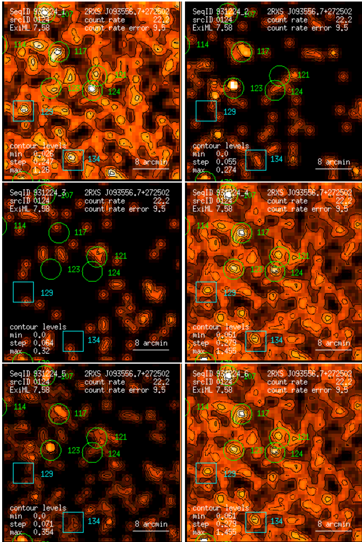
Figure 124: RASS 931224: detection 0124: band rate images, Gaussian filter: (1) PSPC channels 11 – 41, (2) 52 – 90, (3) 91 – 201, (4) 11 – 235, (5) 52 – 201, (6) 11 – 201. Broad band rates in counts/ks. Band rate contour levels in counts/ks/arcmin 2 .
