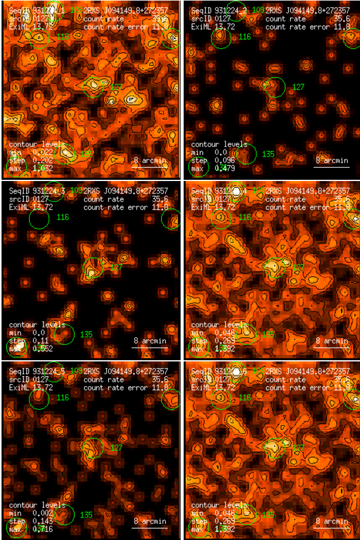
Figure 127: RASS 931224: detection 0127: band rate images, Gaussian filter: (1) PSPC channels 11 – 41, (2) 52 – 90, (3) 91 – 201, (4) 11 – 235, (5) 52 – 201, (6) 11 – 201. Broad band rates in counts/ks. Band rate contour levels in counts/ks/arcmin 2 .
