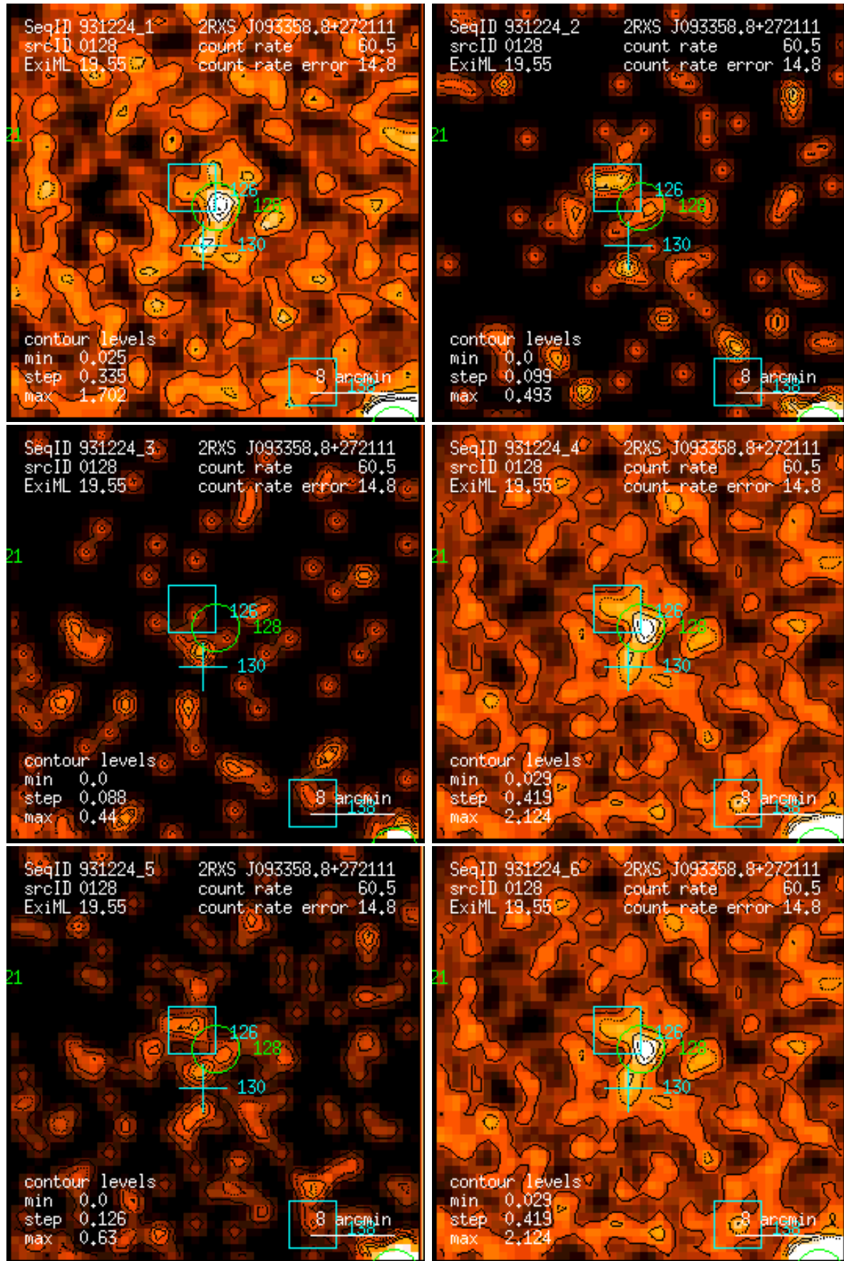
Figure 128: RASS 931224: detection 0128: band rate images, Gaussian filter: (1) PSPC channels 11 – 41, (2) 52 – 90, (3) 91 – 201, (4) 11 – 235, (5) 52 – 201, (6) 11 – 201. Broad band rates in counts/ks. Band rate contour levels in counts/ks/arcmin 2 .
