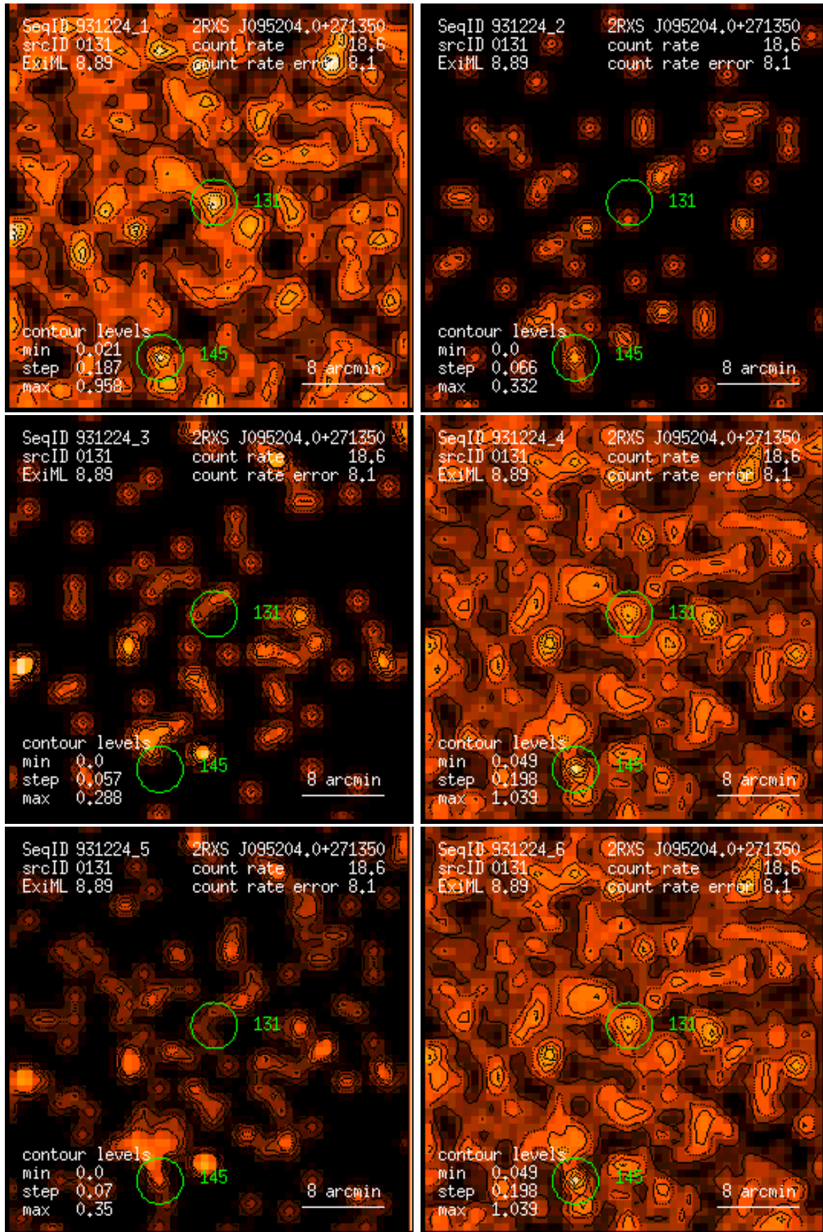
Figure 131: RASS 931224: detection 0131: band rate images, Gaussian filter: (1) PSPC channels 11 – 41, (2) 52 – 90, (3) 91 – 201, (4) 11 – 235, (5) 52 – 201, (6) 11 – 201. Broad band rates in counts/ks. Band rate contour levels in counts/ks/arcmin 2 .
