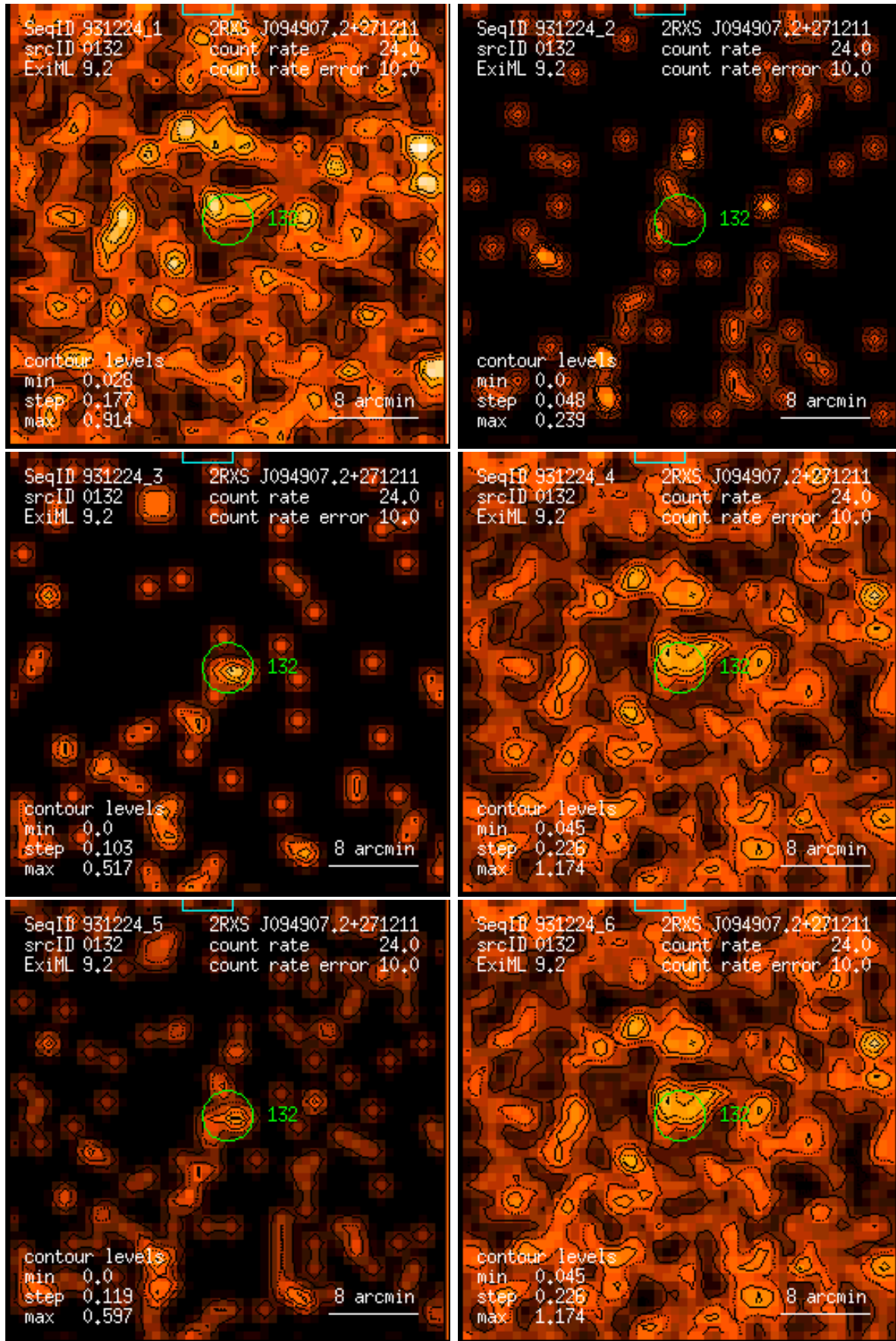
Figure 132: RASS 931224: detection 0132: band rate images, Gaussian filter: (1) PSPC channels 11 – 41, (2) 52 – 90, (3) 91 – 201, (4) 11 – 235, (5) 52 – 201, (6) 11 – 201. Broad band rates in counts/ks. Band rate contour levels in counts/ks/arcmin 2 .
