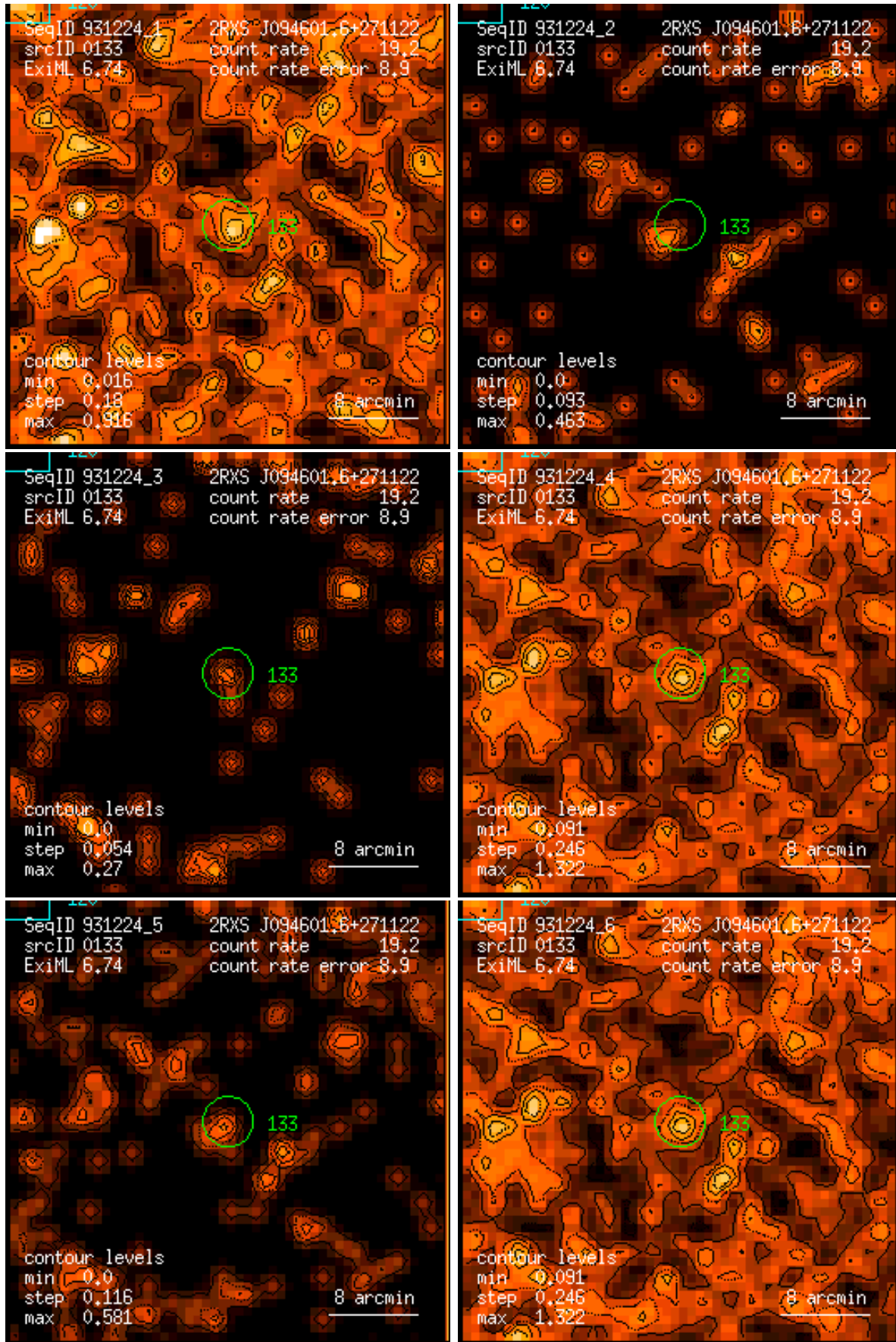
Figure 133: RASS 931224: detection 0133: band rate images, Gaussian filter: (1) PSPC channels 11 – 41, (2) 52 – 90, (3) 91 – 201, (4) 11 – 235, (5) 52 – 201, (6) 11 – 201. Broad band rates in counts/ks. Band rate contour levels in counts/ks/arcmin 2 .
