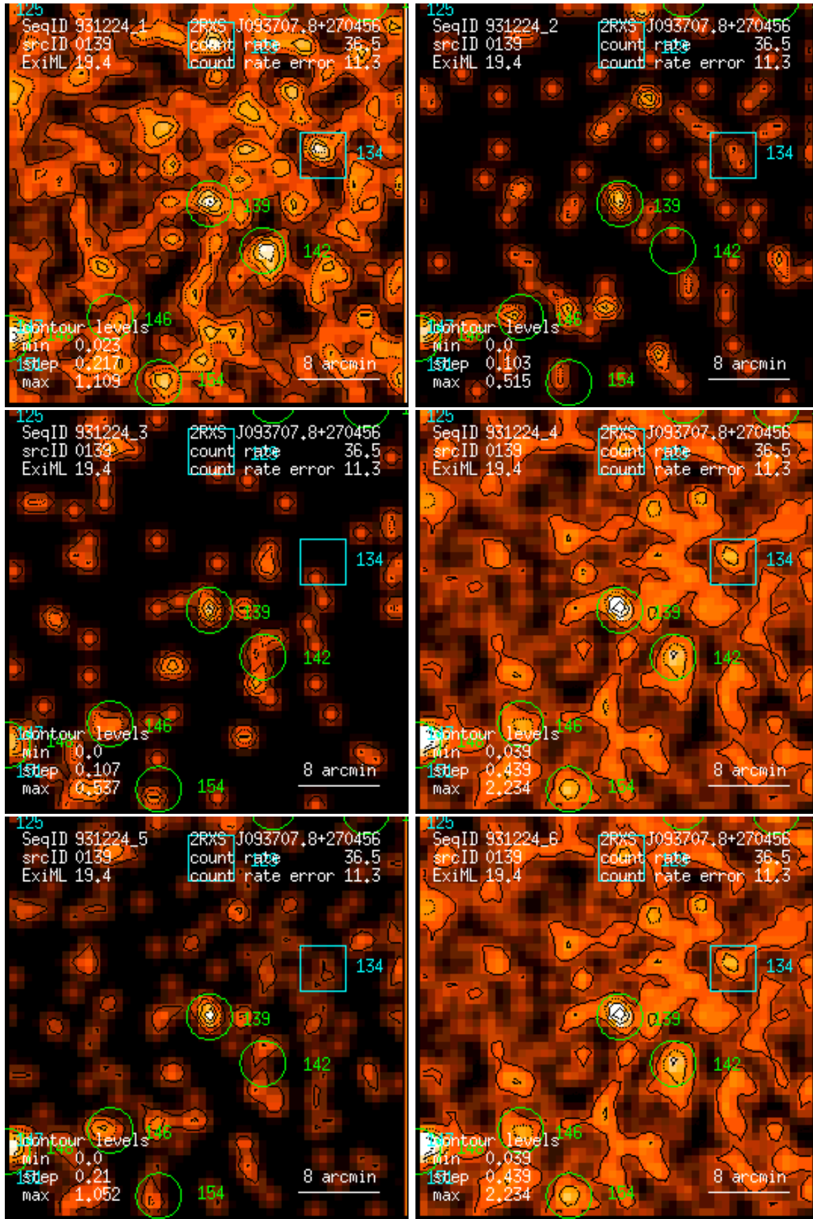
Figure 139: RASS 931224: detection 0139: band rate images, Gaussian filter: (1) PSPC channels 11 – 41, (2) 52 – 90, (3) 91 – 201, (4) 11 – 235, (5) 52 – 201, (6) 11 – 201. Broad band rates in counts/ks. Band rate contour levels in counts/ks/arcmin 2 .
