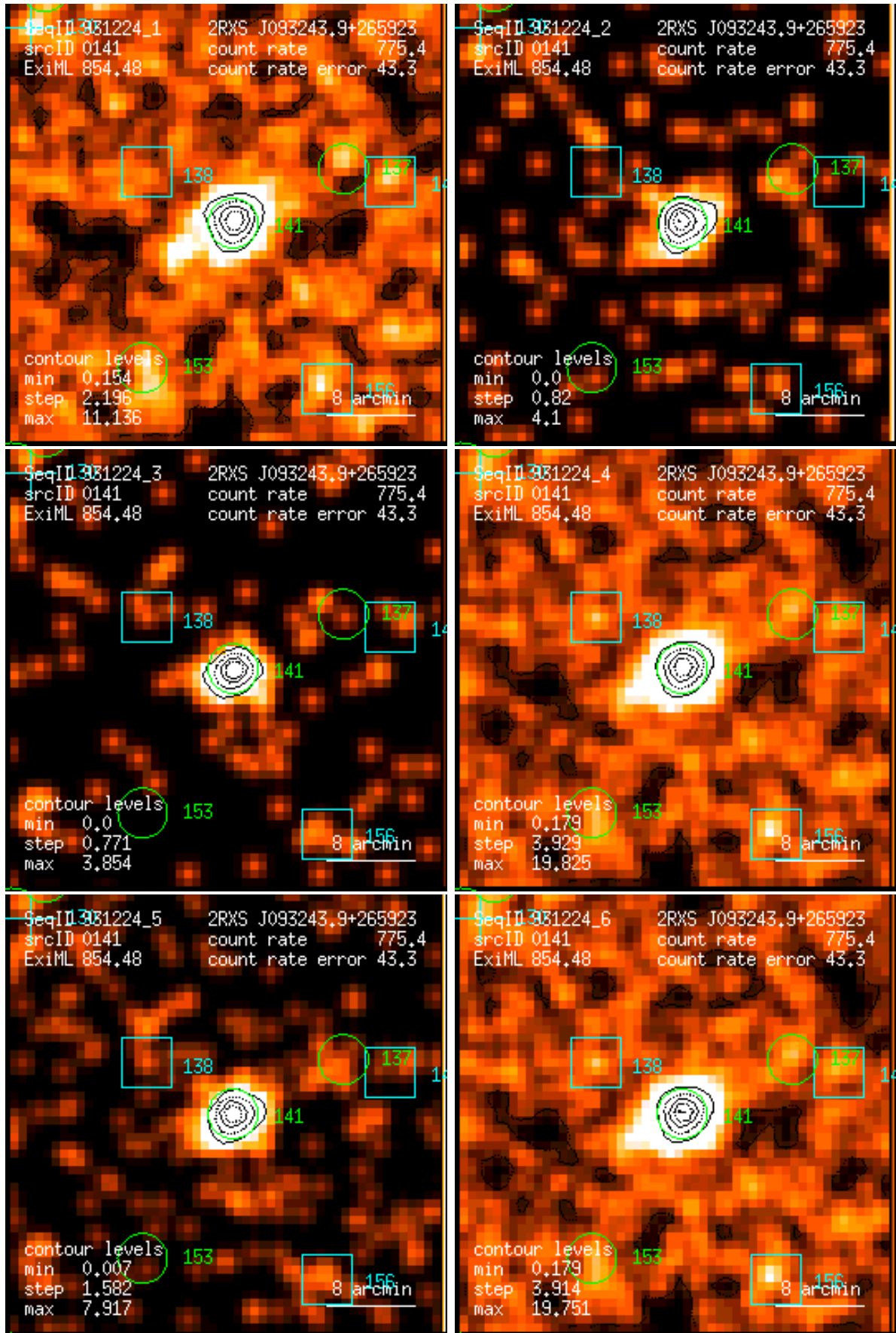
Figure 141: RASS 931224: detection 0141: band rate images, Gaussian filter: (1) PSPC channels 11 – 41, (2) 52 – 90, (3) 91 – 201, (4) 11 – 235, (5) 52 – 201, (6) 11 – 201. Broad band rates in counts/ks. Band rate contour levels in counts/ks/arcmin 2 .
