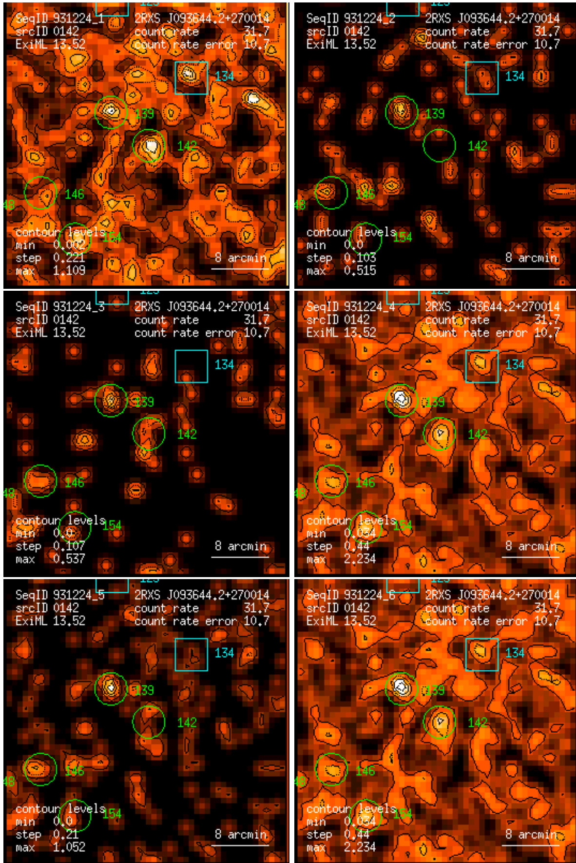
Figure 142: RASS 931224: detection 0142: band rate images, Gaussian filter: (1) PSPC channels 11 – 41, (2) 52 – 90, (3) 91 – 201, (4) 11 – 235, (5) 52 – 201, (6) 11 – 201. Broad band rates in counts/ks. Band rate contour levels in counts/ks/arcmin 2 .
