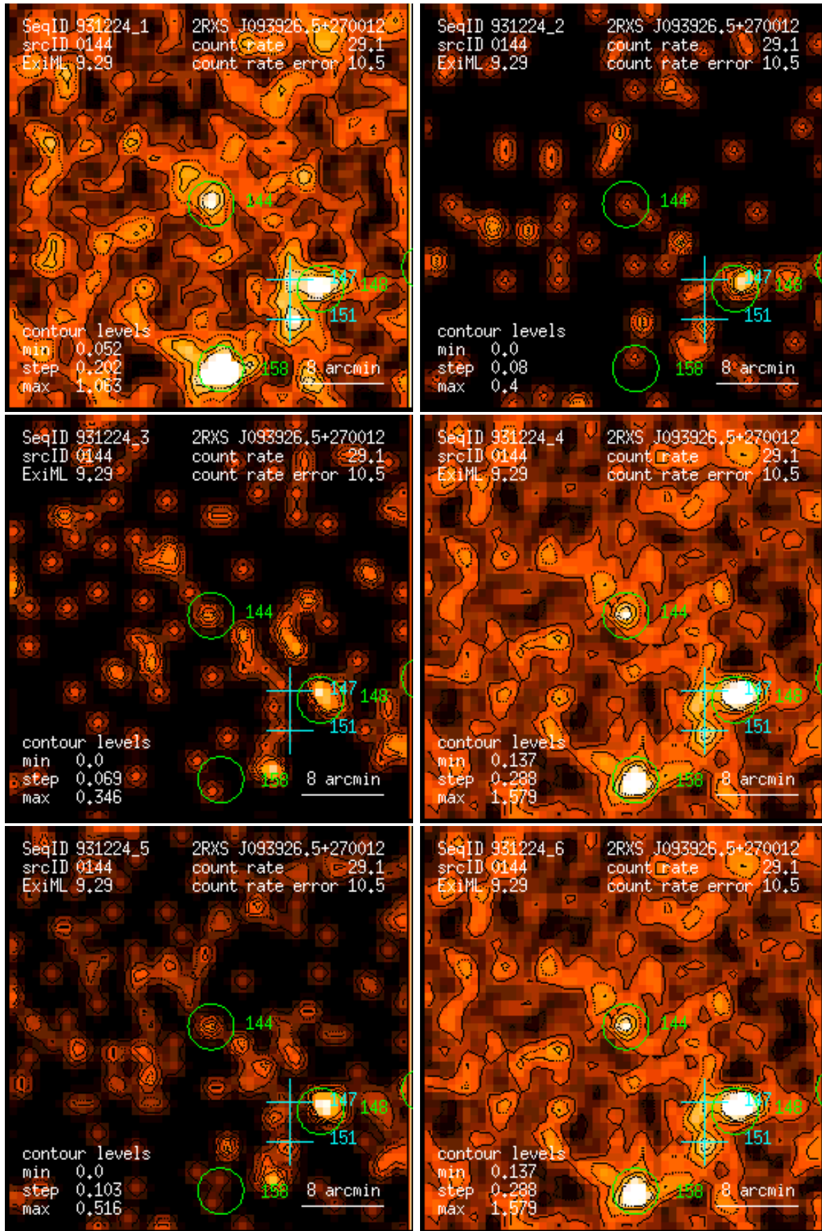
Figure 144: RASS 931224: detection 0144: band rate images, Gaussian filter: (1) PSPPC channels 11 – 41, (2) 52 – 90, (3) 91 – 201, (4) 11 – 235, (5) 52 – 201, (6) 11 – 201. Broad band rates in counts/ks. Band rate contour levels in counts/ks/arcmin 2 .
