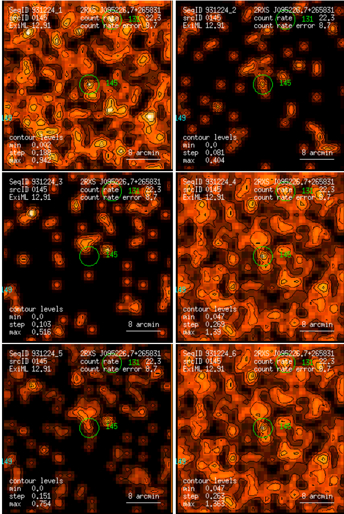
Figure 145: RASS 931224: detection 0145: band rate images, Gaussian filter: (1) PSPC channels 11 – 41, (2) 52 – 90, (3) 91 – 201, (4) 11 – 235, (5) 52 – 201, (6) 11 – 201. Broad band rates in counts/ks. Band rate contour levels in counts/ks/arcmin 2 .
