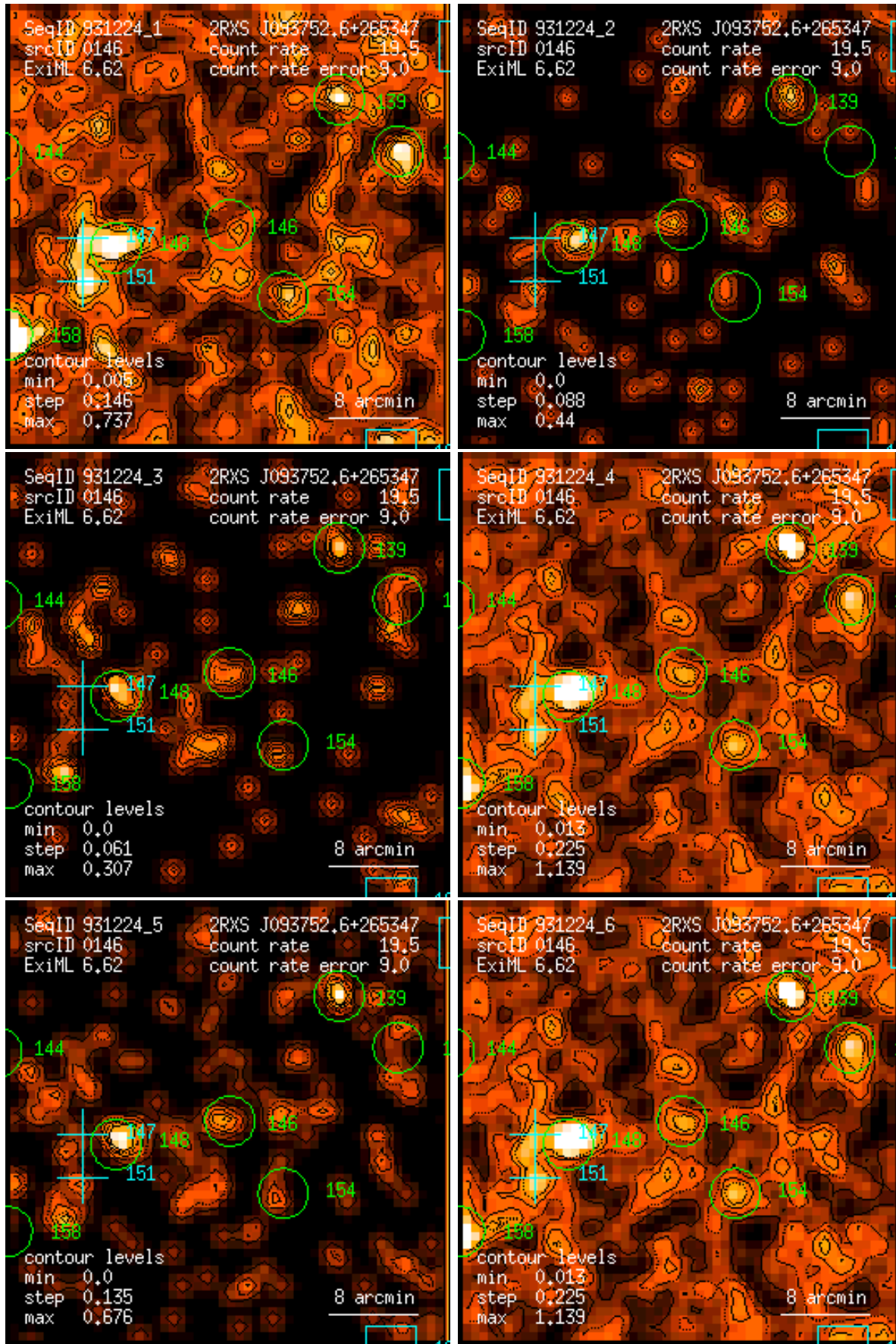
Figure 146: RASS 931224: detection 0146: band rate images, Gaussian filter: (1) PSPC channels 11 – 41, (2) 52 – 90, (3) 91 – 201, (4) 11 – 235, (5) 52 – 201, (6) 11 – 201. Broad band rates in counts/ks. Band rate contour levels in counts/ks/arcmin 2 .
