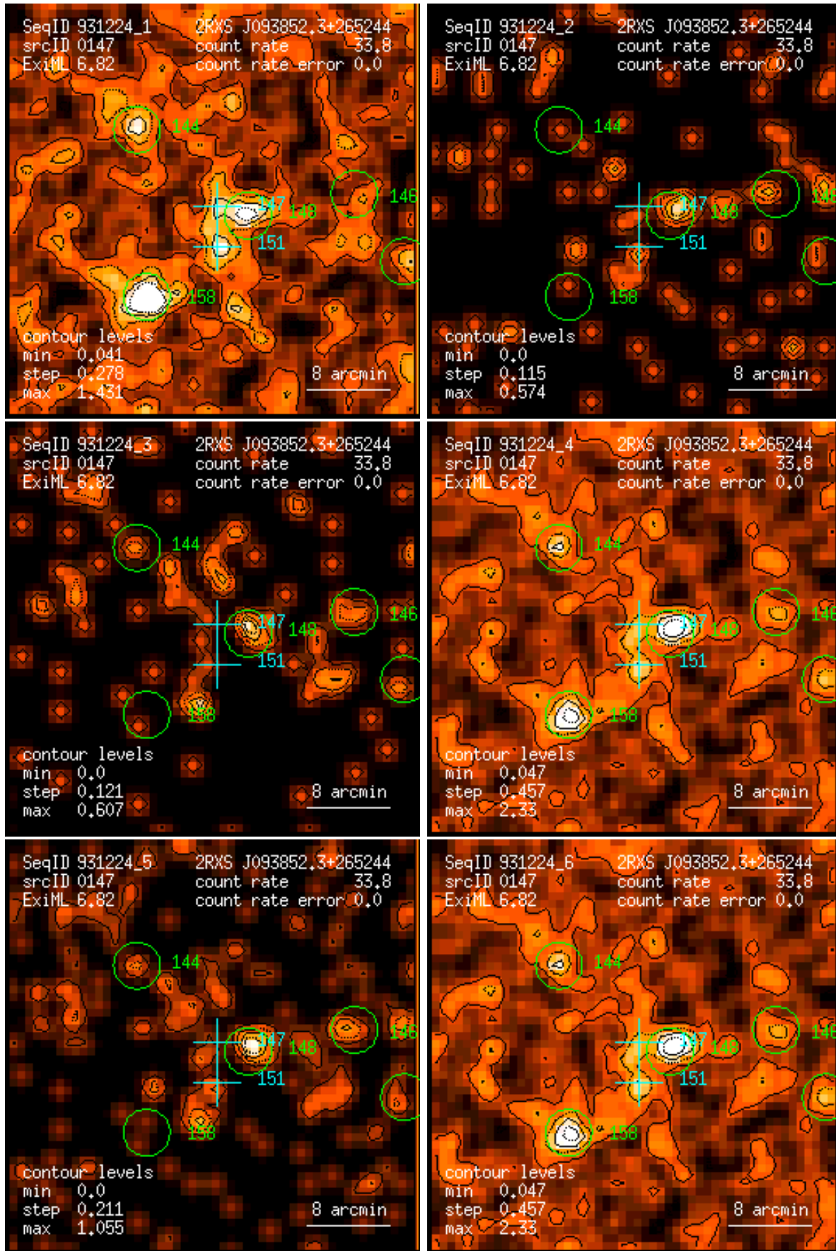
Figure 147: RASS 931224: detection 0147: band rate images, Gaussian filter: (1) PSPC channels 11 – 41, (2) 52 – 90, (3) 91 – 201, (4) 11 – 235, (5) 52 – 201, (6) 11 – 201. Broad band rates in counts/ks. Band rate contour levels in counts/ks/arcmin 2 .
