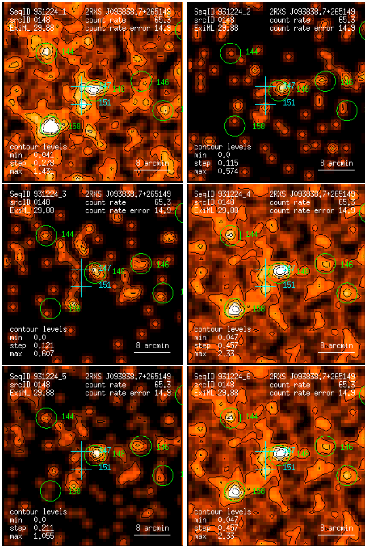
Figure 148: RASS 931224: detection 0148: band rate images, Gaussian filter: (1) PSPC channels 11 – 41, (2) 52 – 90, (3) 91 – 201, (4) 11 – 235, (5) 52 – 201, (6) 11 – 201. Broad band rates in counts/ks. Band rate contour levels in counts/ks/arcmin 2 .
