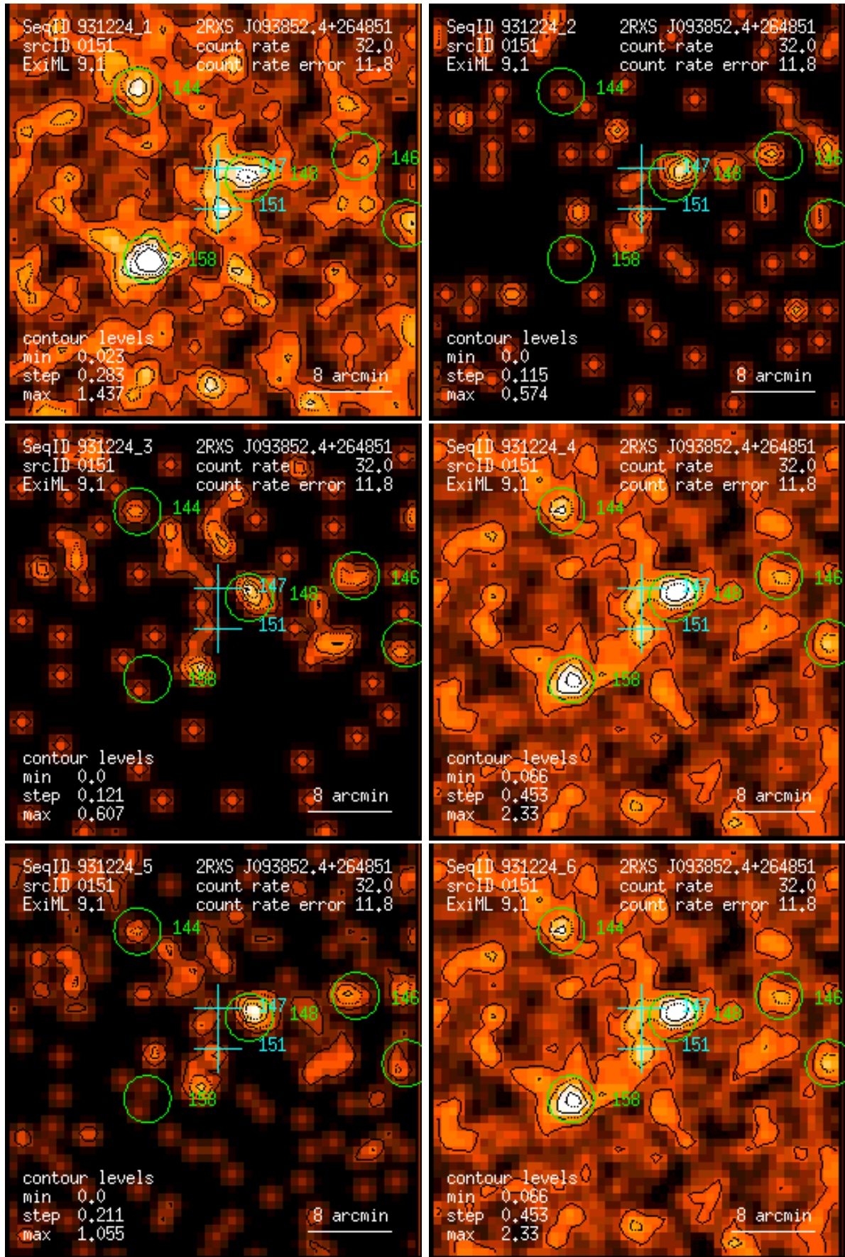
Figure 151: RASS 931224: detection 0151: band rate images, Gaussian filter: (1) PSPC channels 11 – 41, (2) 52 – 90, (3) 91 – 201, (4) 11 – 235, (5) 52 – 201, (6) 11 – 201. Broad band rates in counts/ks. Band rate contour levels in counts/ks/arcmin 2 .
