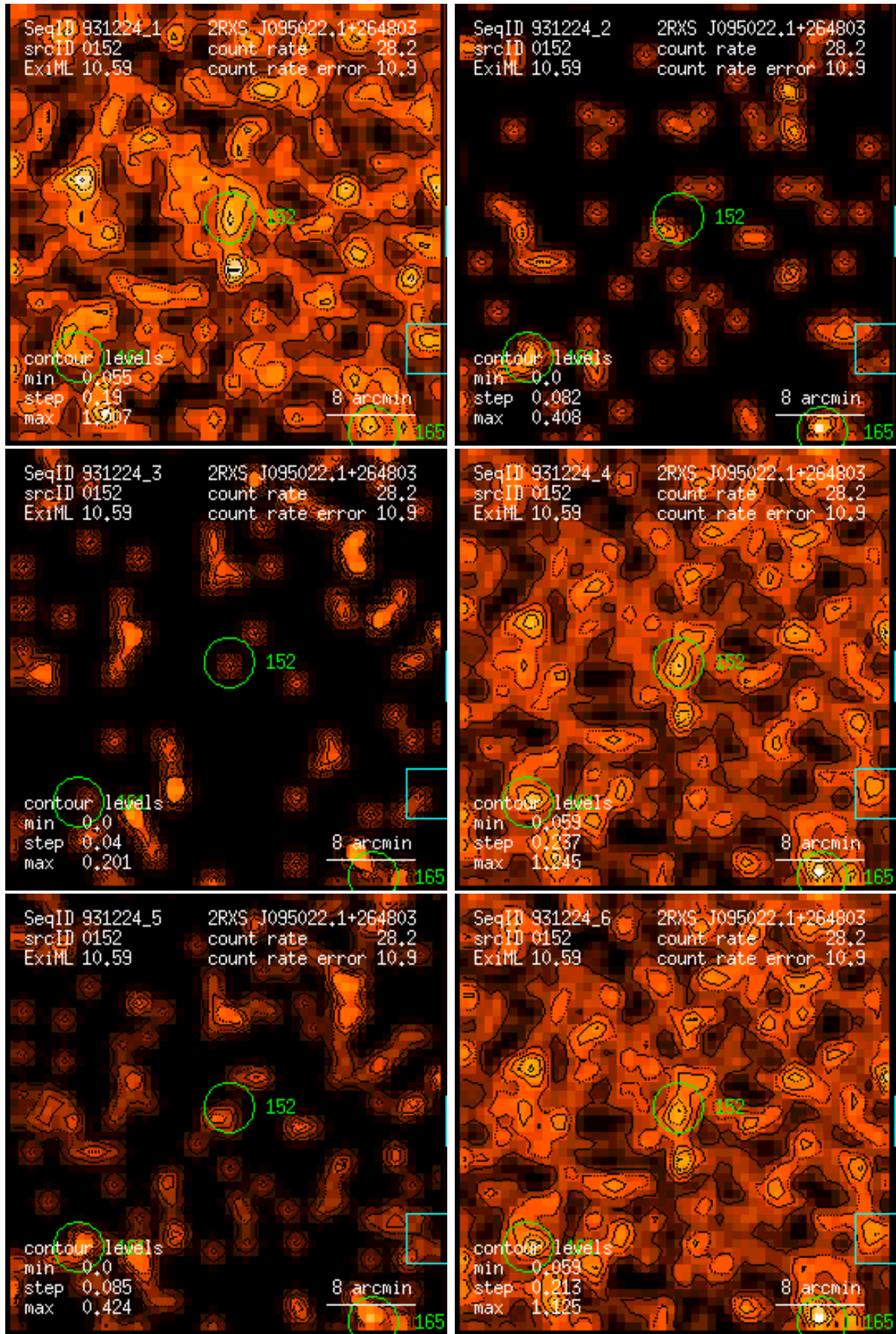
Figure 152: RASS 931224: detection 0152: band rate images, Gaussian filter: (1) PSPC channels 11 – 41, (2) 52 – 90, (3) 91 – 201, (4) 11 – 235, (5) 52 – 201, (6) 11 – 201. Broad band rates in counts/ks. Band rate contour levels in counts/ks/arcmin 2 .
