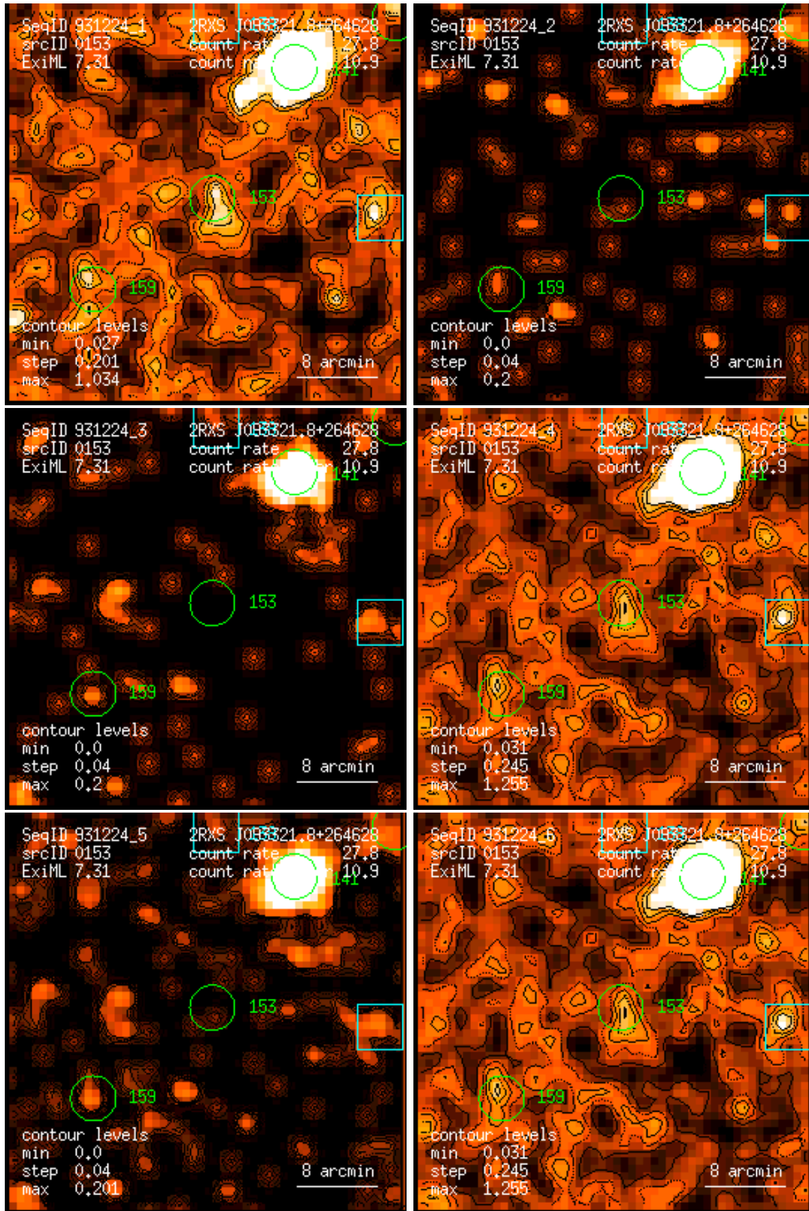
Figure 153: RASS 931224: detection 0153: band rate images, Gaussian filter: (1) PSPC channels 11 – 41, (2) 52 – 90, (3) 91 – 201, (4) 11 – 235, (5) 52 – 201, (6) 11 – 201. Broad band rates in counts/ks. Band rate contour levels in counts/ks/arcmin 2 .
