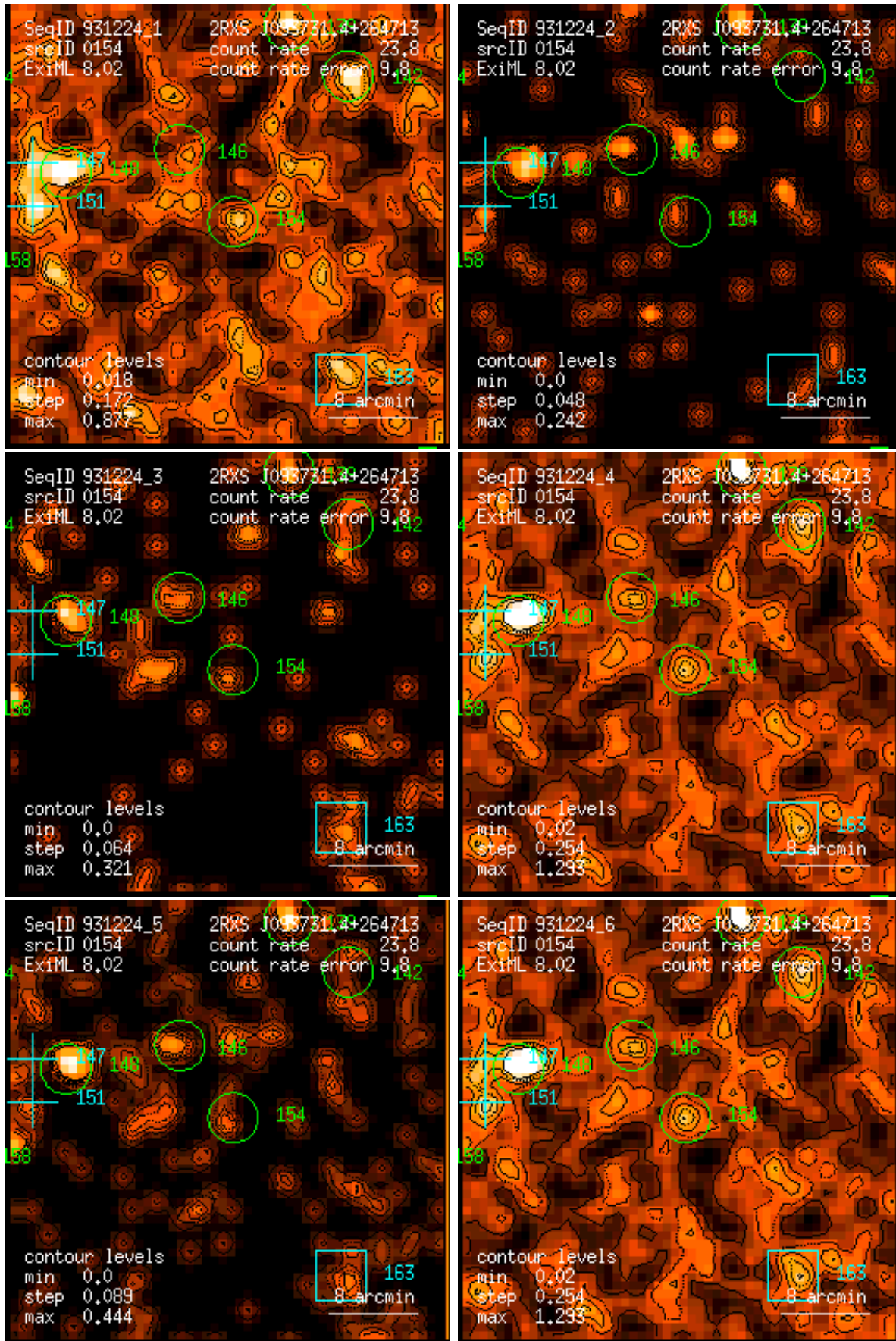
Figure 154: RASS 931224: detection 0154: band rate images, Gaussian filter: (1) PSPC channels 11 – 41, (2) 52 – 90, (3) 91 – 201, (4) 11 – 235, (5) 52 – 201, (6) 11 – 201. Broad band rates in counts/ks. Band rate contour levels in counts/ks/arcmin 2 .
