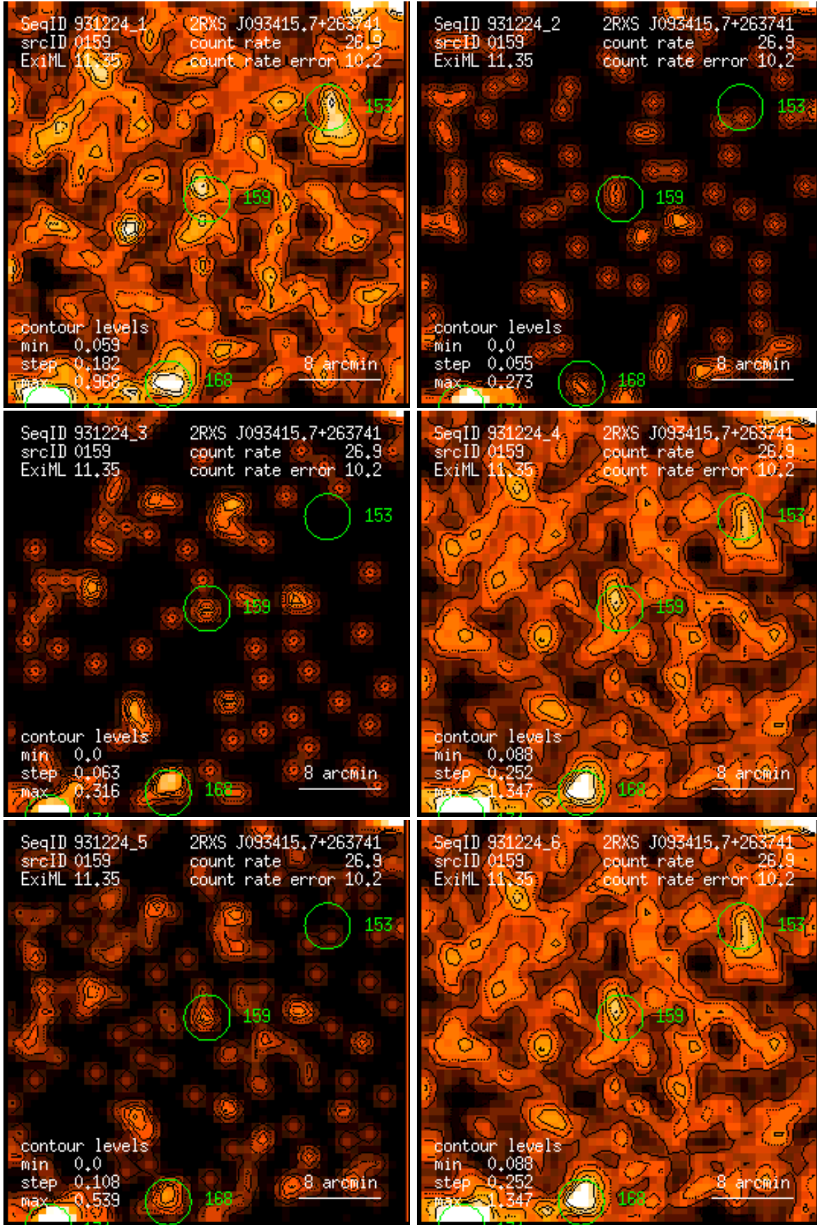
Figure 159: RASS 931224: detection 0159: band rate images, Gaussian filter: (1) PSPC channels 11 – 41, (2) 52 – 90, (3) 91 – 201, (4) 11 – 235, (5) 52 – 201, (6) 11 – 201. Broad band rates in counts/ks. Band rate contour levels in counts/ks/arcmin 2 .
