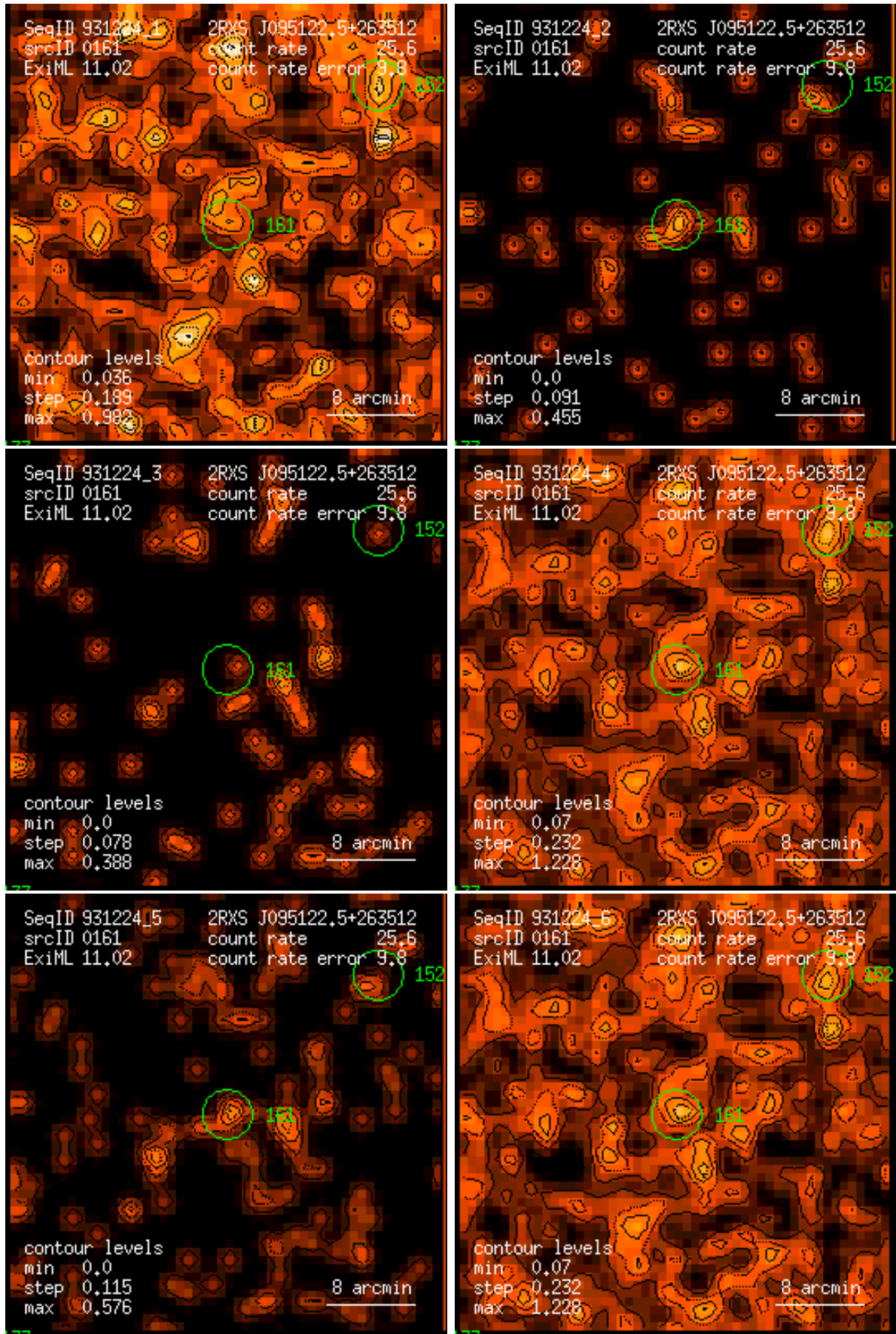
Figure 161: RASS 931224: detection 0161: band rate images, Gaussian filter: (1) PSPC channels 11 – 41, (2) 52 – 90, (3) 91 – 201, (4) 11 – 235, (5) 52 – 201, (6) 11 – 201. Broad band rates in counts/ks. Band rate contour levels in counts/ks/arcmin 2 .
