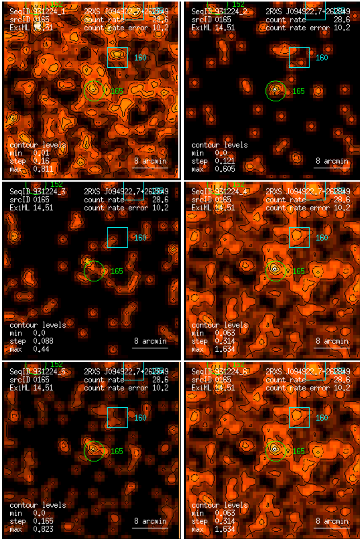
Figure 165: RASS 931224: detection 0165: band rate images, Gaussian filter: (1) PSPC channels 11 – 41, (2) 52 – 90, (3) 91 – 201, (4) 11 – 235, (5) 52 – 201, (6) 11 – 201. Broad band rates in counts/ks. Band rate contour levels in counts/ks/arcmin 2 .
