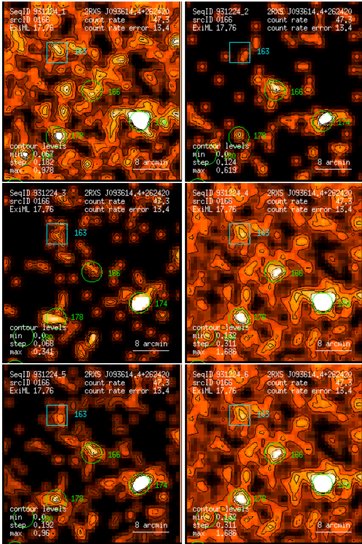
Figure 166: RASS 931224: detection 0166: band rate images, Gaussian filter: (1) PSPC channels 11 – 41, (2) 52 – 90, (3) 91 – 201, (4) 11 – 235, (5) 52 – 201, (6) 11 – 201. Broad band rates in counts/ks. Band rate contour levels in counts/ks/arcmin 2 .
