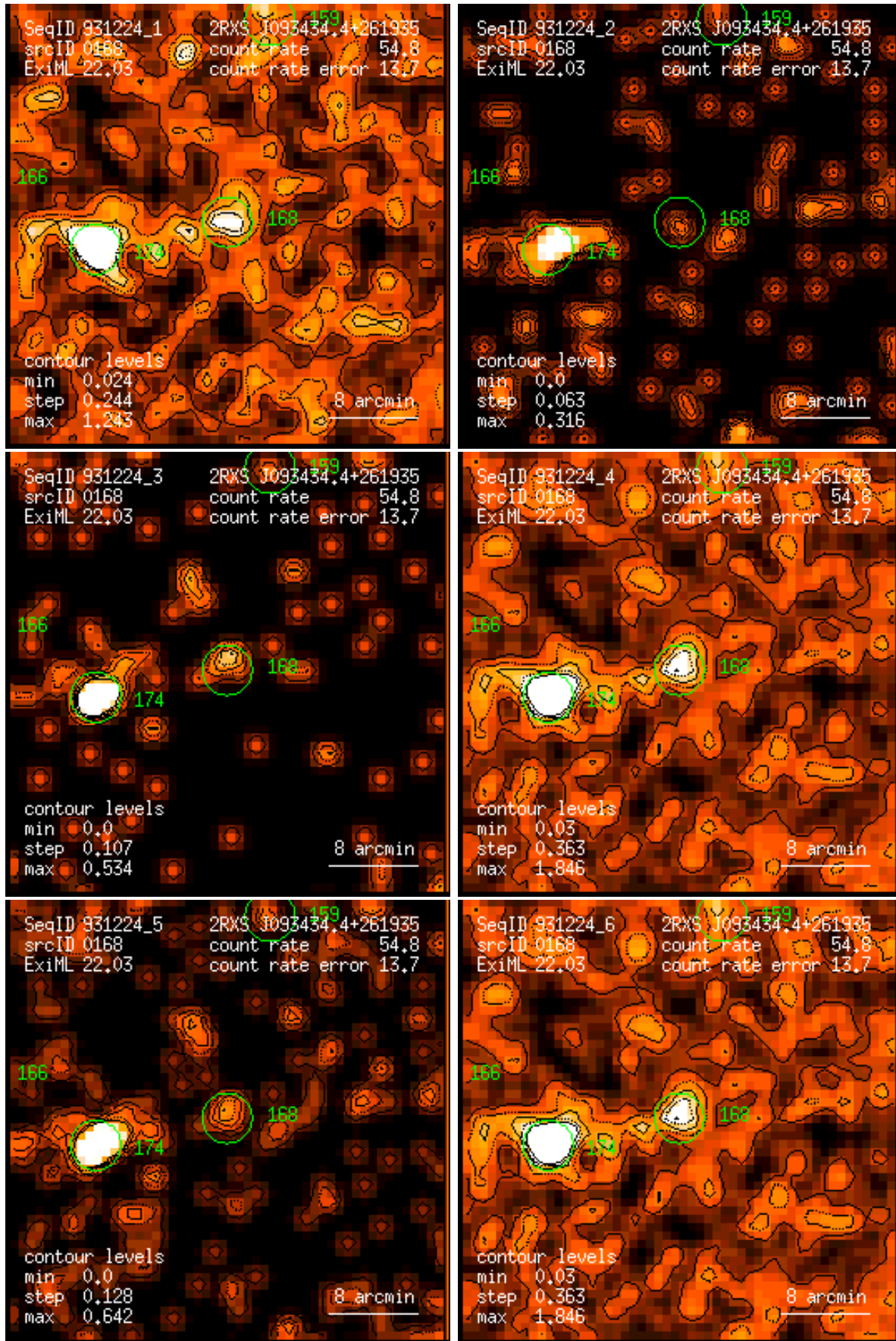
Figure 168: RASS 931224: detection 0168: band rate images, Gaussian filter: (1) PSPC channels 11 – 41, (2) 52 – 90, (3) 91 – 201, (4) 11 – 235, (5) 52 – 201, (6) 11 – 201. Broad band rates in counts/ks. Band rate contour levels in counts/ks/arcmin 2 .
