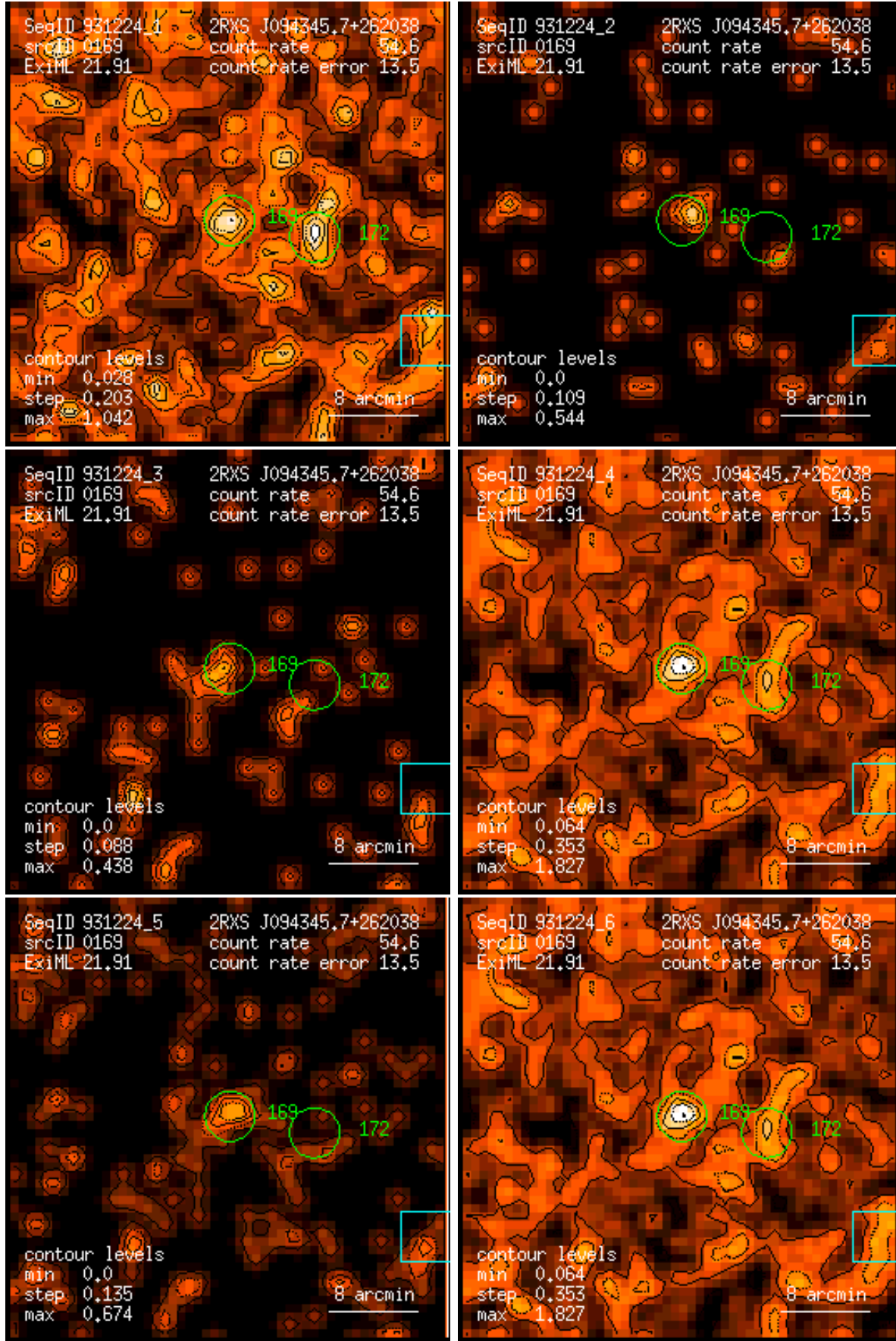
Figure 169: RASS 931224: detection 0169: band rate images, Gaussian filter: (1) PSPC channels 11 – 41, (2) 52 – 90, (3) 91 – 201, (4) 11 – 235, (5) 52 – 201, (6) 11 – 201. Broad band rates in counts/ks. Band rate contour levels in counts/ks/arcmin 2 .
