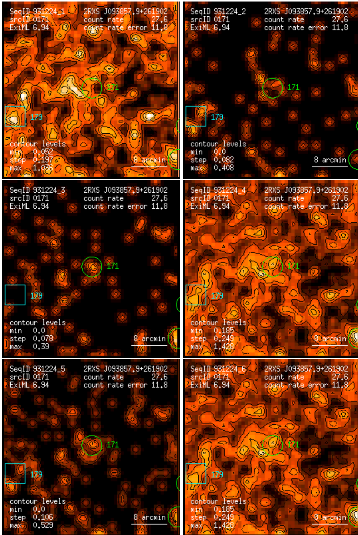
Figure 171: RASS 931224: detection 0171: band rate images, Gaussian filter: (1) PSPC channels 11 – 41, (2) 52 – 90, (3) 91 – 201, (4) 11 – 235, (5) 52 – 201, (6) 11 – 201. Broad band rates in counts/ks. Band rate contour levels in counts/ks/arcmin 2 .
