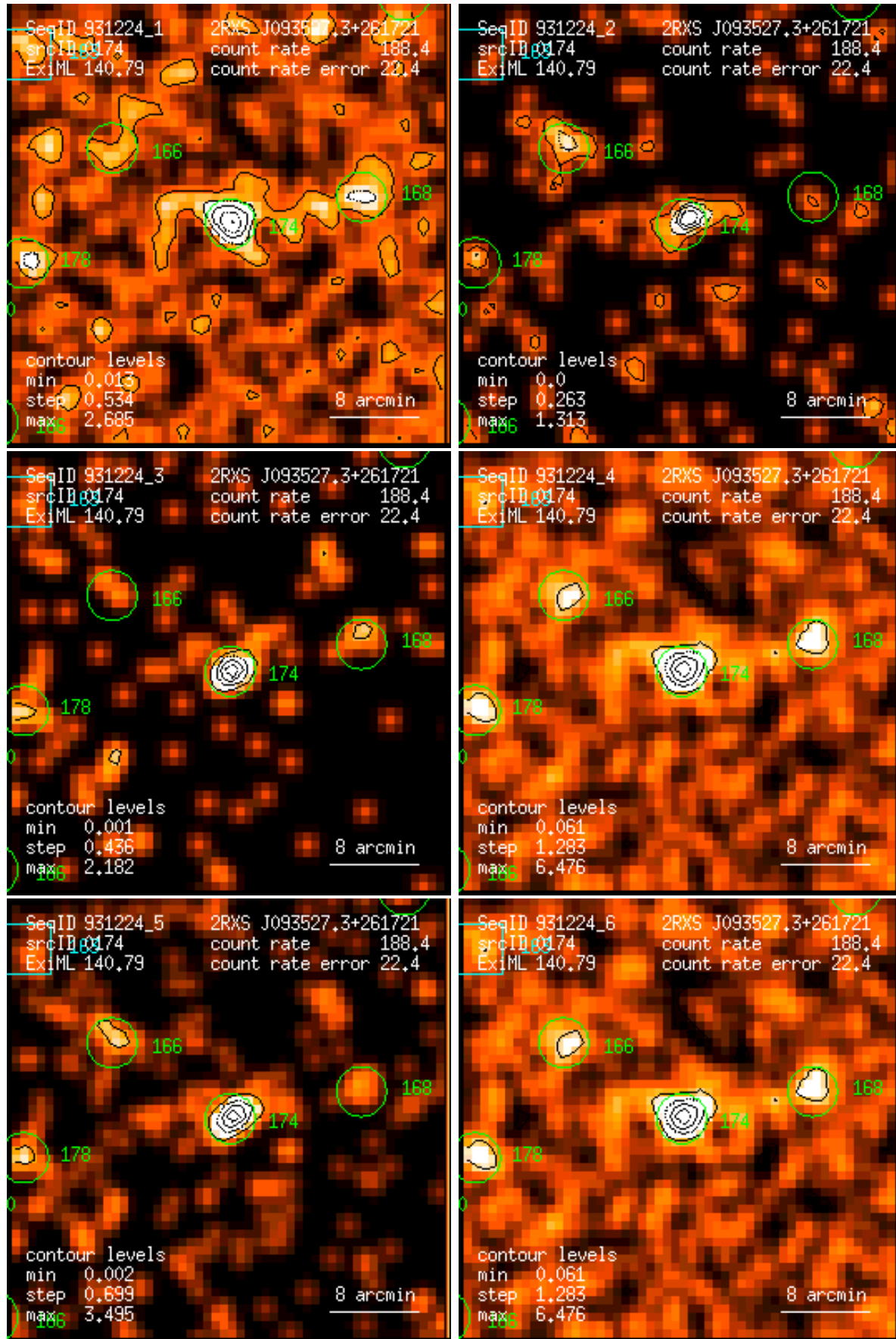
Figure 174: RASS 931224: detection 0174: band rate images, Gaussian filter: (1) PSPC channels 11 – 41, (2) 52 – 90, (3) 91 – 201, (4) 11 – 235, (5) 52 – 201, (6) 11 – 201. Broad band rates in counts/ks. Band rate contour levels in counts/ks/arcmin 2 .
