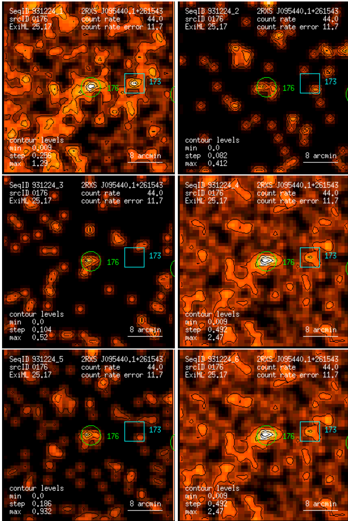
Figure 176: RASS 931224: detection 0176: band rate images, Gaussian filter: (1) PSPC channels 11 – 41, (2) 52 – 90, (3) 91 – 201, (4) 11 – 235, (5) 52 – 201, (6) 11 – 201. Broad band rates in counts/ks. Band rate contour levels in counts/ks/arcmin 2 .
