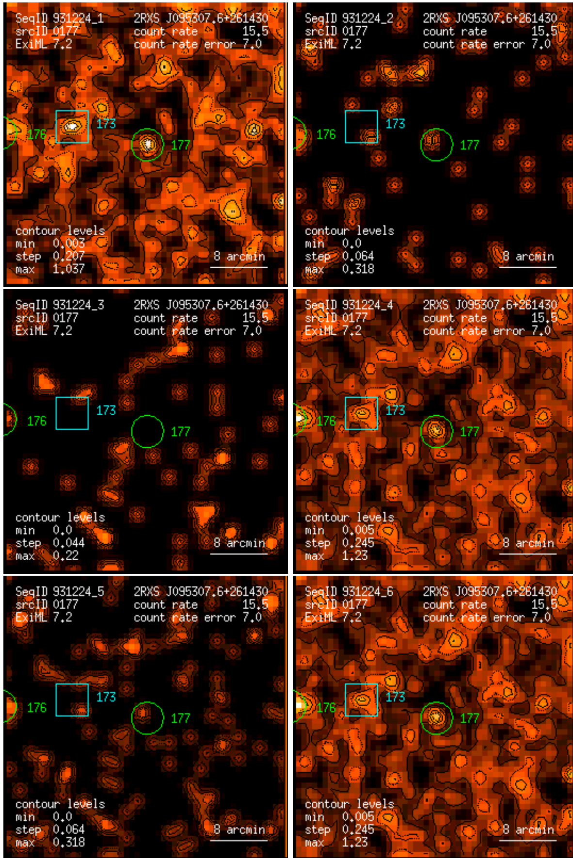
Figure 177: RASS 931224: detection 0177: band rate images, Gaussian filter: (1) PSPPC channels 11 – 41, (2) 52 – 90, (3) 91 – 201, (4) 11 – 235, (5) 52 – 201, (6) 11 – 201. Broad band rates in counts/ks. Band rate contour levels in counts/ks/arcmin 2 .
