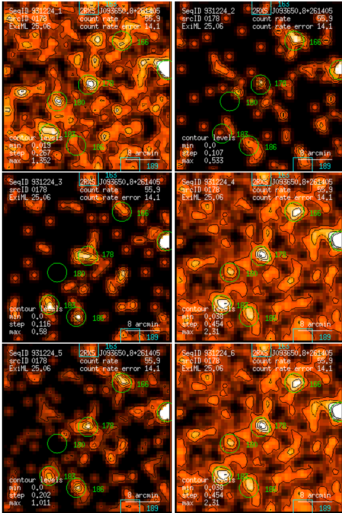
Figure 178: RASS 931224: detection 0178: band rate images, Gaussian filter: (1) PSPC channels 11 – 41, (2) 52 – 90, (3) 91 – 201, (4) 11 – 235, (5) 52 – 201, (6) 11 – 201. Broad band rates in counts/ks. Band rate contour levels in counts/ks/arcmin 2 .
