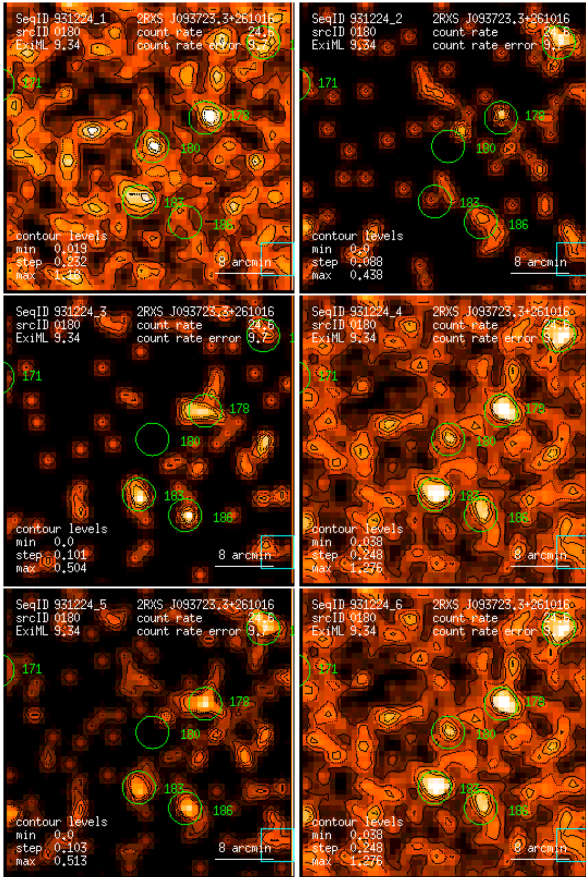
Figure 180: RASS 931224: detection 0180: band rate images, Gaussian filter: (1) PSPC channels 11 – 41, (2) 52 – 90, (3) 91 – 201, (4) 11 – 235, (5) 52 – 201, (6) 11 – 201. Broad band rates in counts/ks. Band rate contour levels in counts/ks/arcmin 2 .
