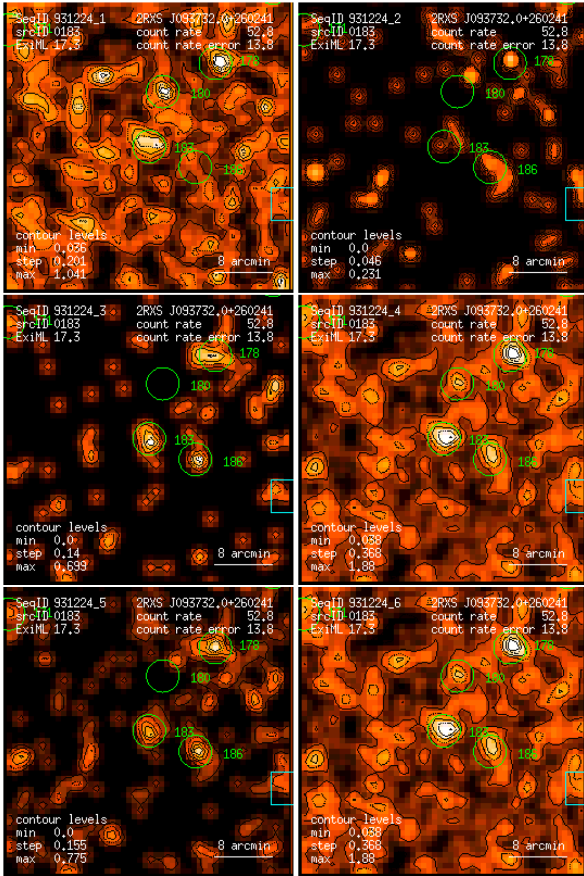
Figure 183: RASS 931224: detection 0183: band rate images, Gaussian filter: (1) PSPC channels 11 – 41, (2) 52 – 90, (3) 91 – 201, (4) 11 – 235, (5) 52 – 201, (6) 11 – 201. Broad band rates in counts/ks. Band rate contour levels in counts/ks/arcmin 2 .
