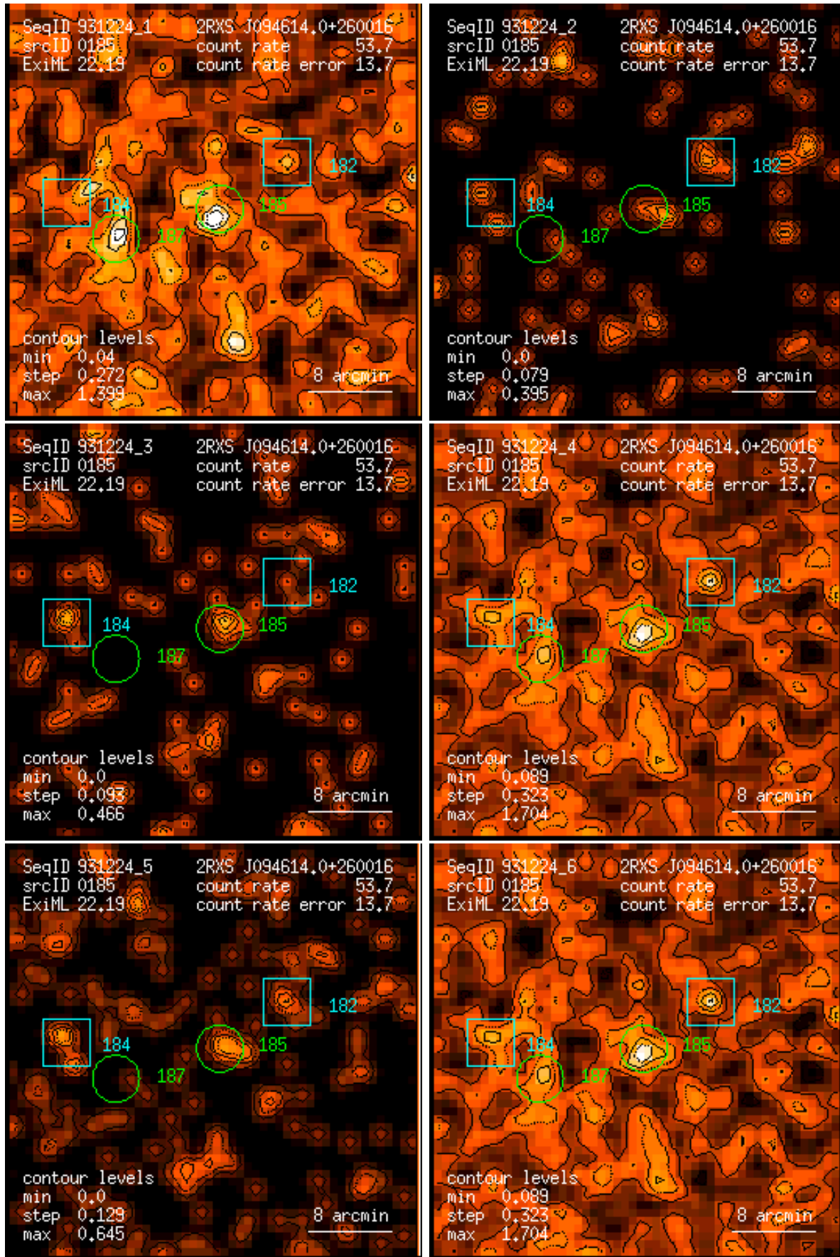
Figure 185: RASS 931224: detection 0185: band rate images, Gaussian filter: (1) PSPC channels 11 – 41, (2) 52 – 90, (3) 91 – 201, (4) 11 – 235, (5) 52 – 201, (6) 11 – 201. Broad band rates in counts/ks. Band rate contour levels in counts/ks/arcmin 2 .
