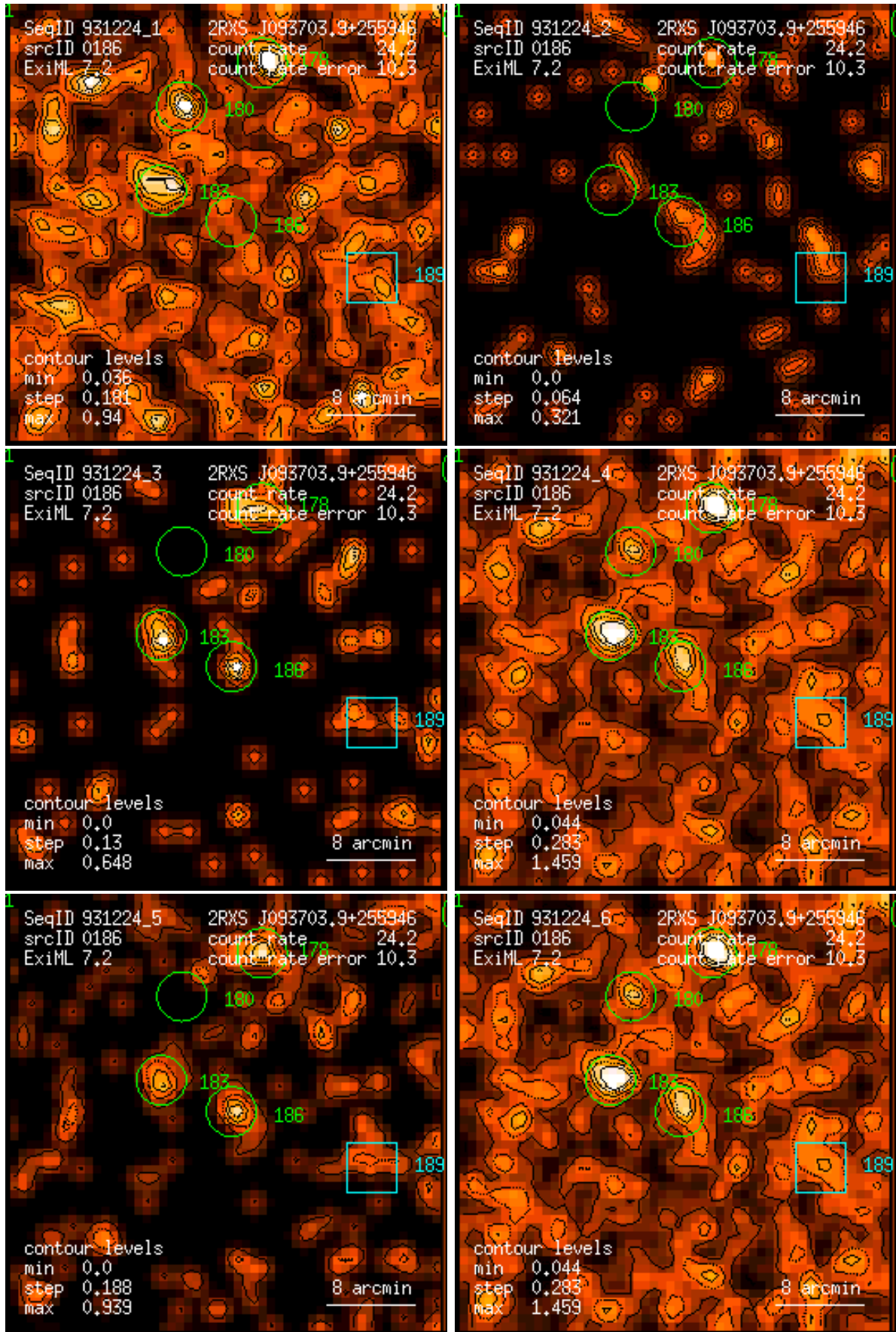
Figure 186: RASS 931224: detection 0186: band rate images, Gaussian filter: (1) PSPC channels 11 – 41, (2) 52 – 90, (3) 91 – 201, (4) 11 – 235, (5) 52 – 201, (6) 11 – 201. Broad band rates in counts/ks. Band rate contour levels in counts/ks/arcmin 2 .
