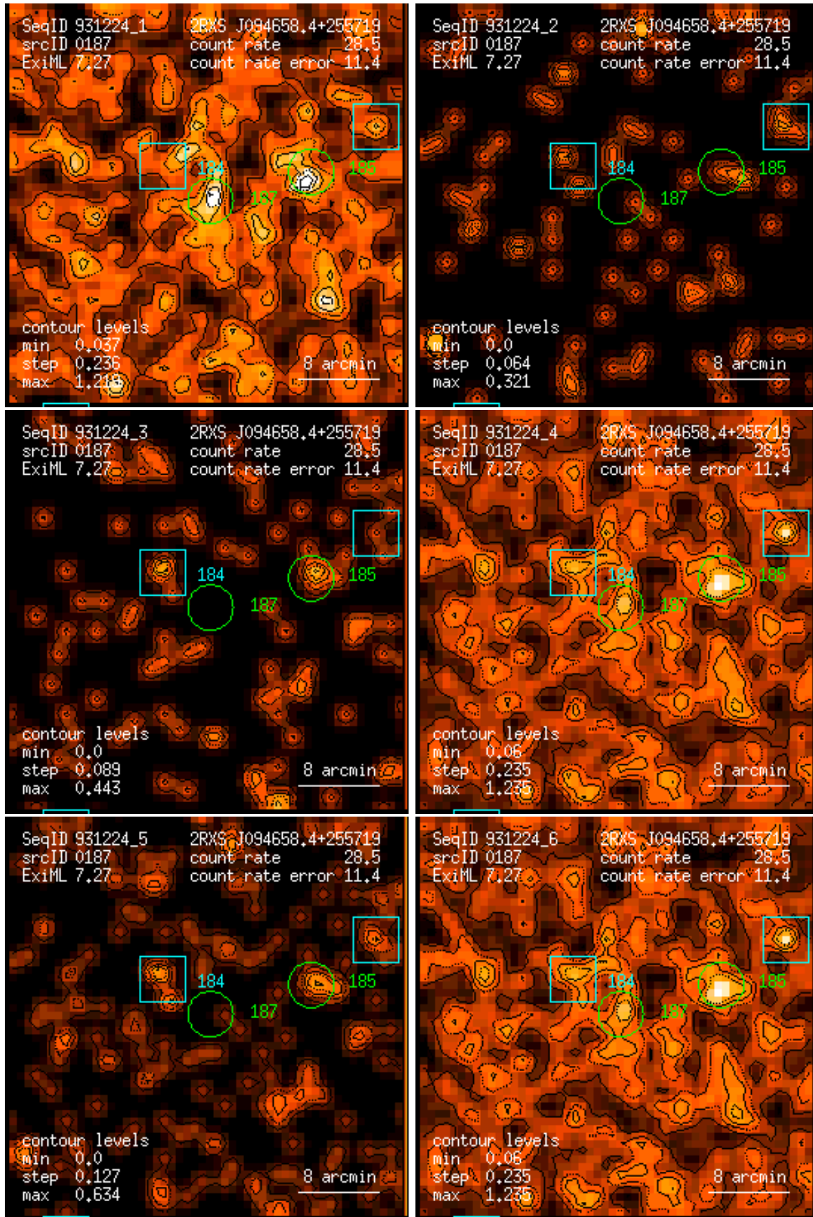
Figure 187: RASS 931224: detection 0187: band rate images, Gaussian filter: (1) PSPC channels 11 – 41, (2) 52 – 90, (3) 91 – 201, (4) 11 – 235, (5) 52 – 201, (6) 11 – 201. Broad band rates in counts/ks. Band rate contour levels in counts/ks/arcmin 2 .
